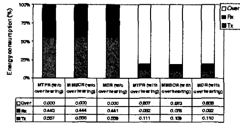
Fig. 3. Static environment scenario: energy consumption.
