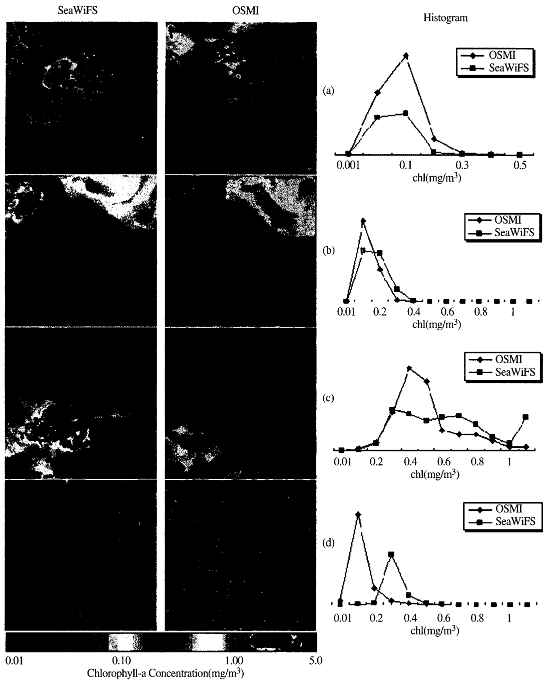
Fig. 2. OSMI-retrieved chlorophyll-a concentration compared to those derived from SeaWiFS measurements for (a) BATS_1 (5 April 2002), (b) BATS_2 (28 April 2001), (c) Galapagos (4 April 2001), (d) HOT (22 May 2001).
