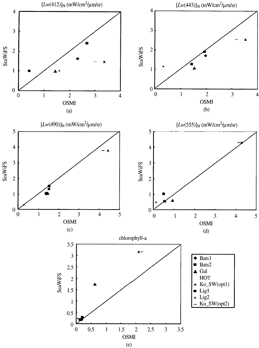
Fig. 1. OSMI-derived normalized water-leaving radiance and chlorophyll-a concentration compared to those of the SeaWiFS: (a) nLw 412 nm (b) nLw 443 nm (c) nLw 490 nm (d) nLw 555 nm (e) chlorophyll-a.
