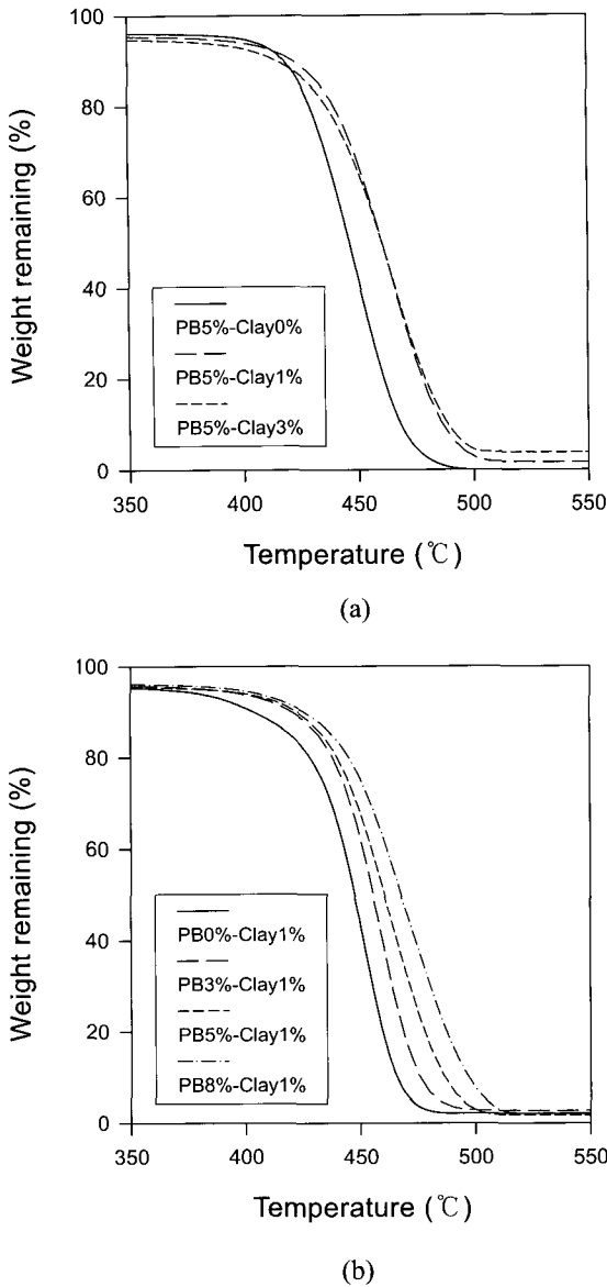
Figure 7. TGA thermograms of HIPS/OLS nanocomposites: (a) effect of clay content and (b) effect of rubber content.
