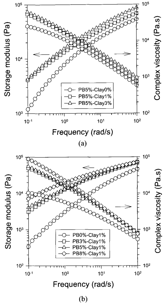
Figure 8. Rheological properties of HIPS/OLS nanocomposites: (a) effect of clay content and (b) effect of rubber content.
