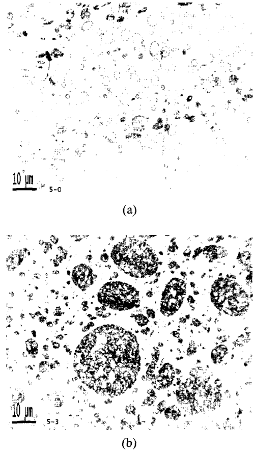
Figure 5. TEM micrographs of samples prepared for the effect of clay addition: (a) HIPS (PB5%-Clay0%) and (b) HIPS/OLS (PB5%-Clay3%).
