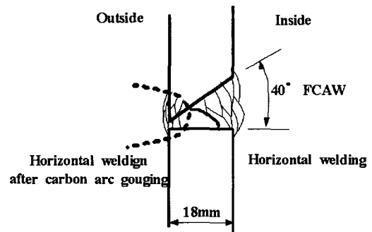
Fig. 3 Schematic diagram of previous used horizontal welding process
