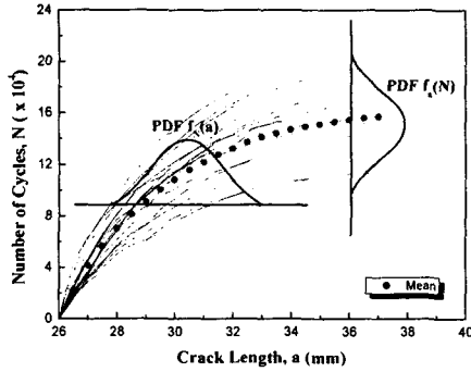
Fig. 1 Crack growth curves for the sixteen specimens studied
