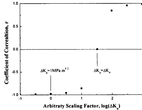
Fig. 9 Dependence of the coefficient of correlation between \log C_n and m on the scaling factor, \Delta K_n
