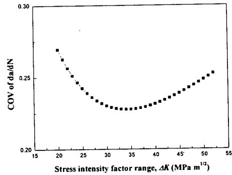
Fig. 7 Coefficients of variation (COV) of da/dN for stress intensity factor range, \Delta K
