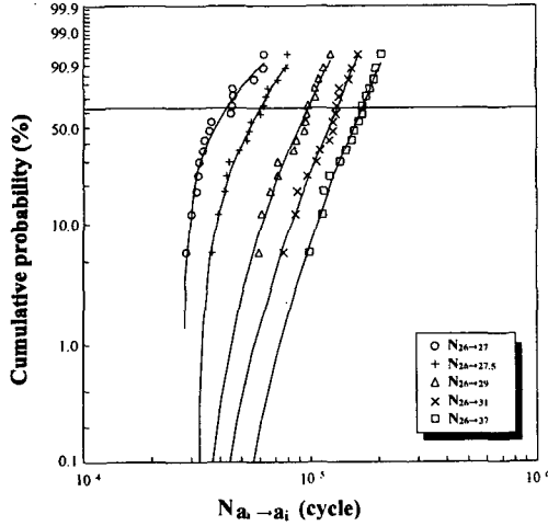
Fig. 3 3-parameter Weibull plots for the various crack growth life, N_{a_0 \to a_i} .
