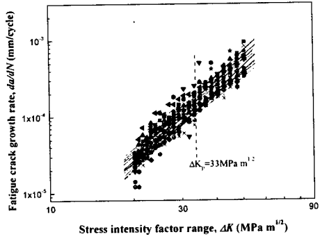
Fig. 4 Relation between da/dN and \Delta K
