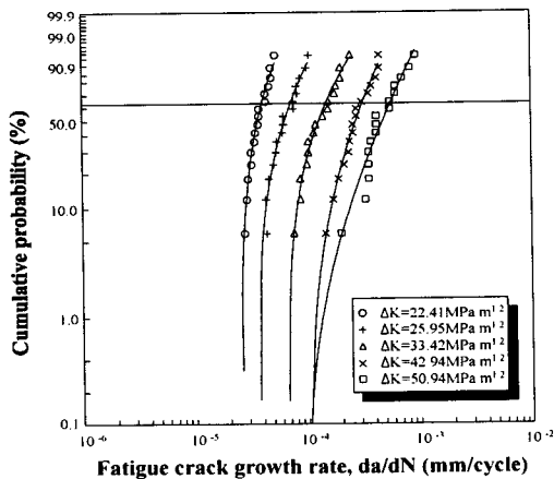
Fig. 6 3-parameter Weibull plots of fatigue crack growth rate, da/dN
