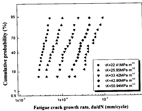
Fig. 5 Log-normal plots of fatigue crack growth rate, da/dN
