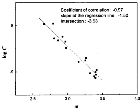
Fig. 8 Scatterplot of the values of \log C and m
