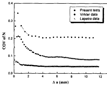
Fig. 2 Coefficients of variation (COV) of fatigue crack growth life for incremental crack length, \Delta a = a_0 - a_i
