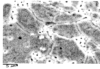
(c) 15 mol.%
