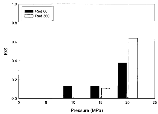
Fig. 7. Relationship between dyeing property and pressure in supercritical fluid dyeing (130°C × 60min, 0.5% o.w.f. of dyes).
