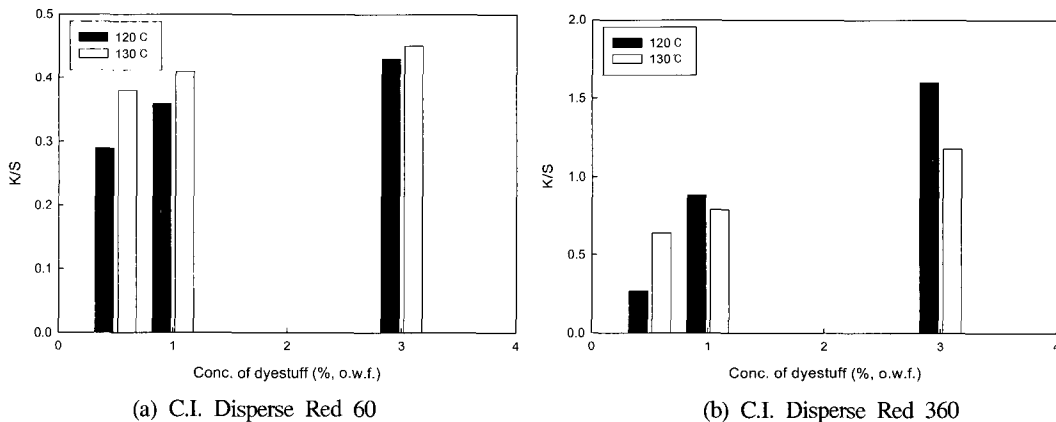
Fig. 4. Relationship between temperature and concentration of dyes in supercritical fluid dyeing(20MPa × 60min).
