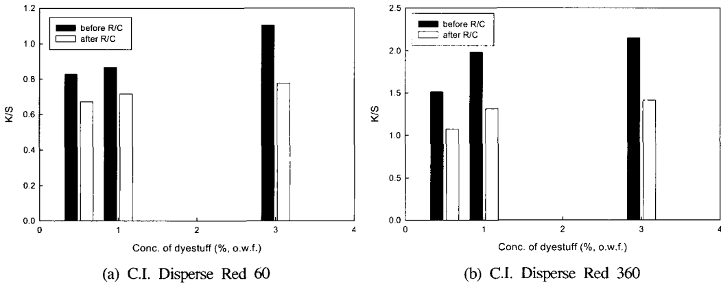
Fig. 6. Relationship between dyeing ability and before and after R/C in wet dyeing (130°C × 60min).
