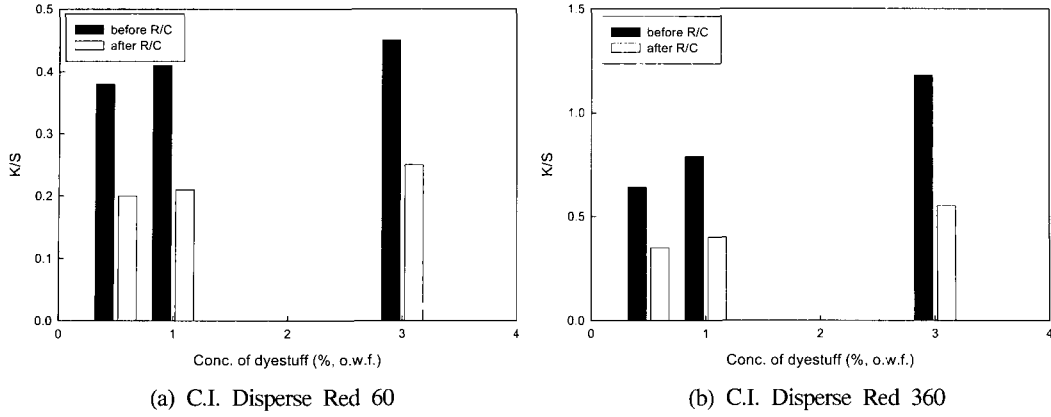
Fig. 5. Relationship between dyeing ability and before and after R/C in supercritical fluid dyeing (130°C × 20MPa × 60min).
