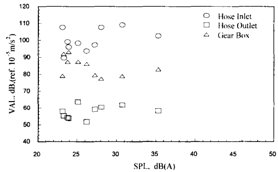
Fig. 7 The variations of the 1st order vibration acceleration level with the 1 st order sound pressure level of interior noise
