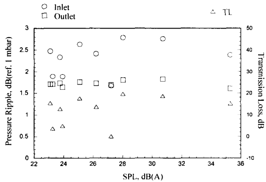
Fig. 8 The variations of the 1st order pressure ripple peak levels and transmission loss with the 1 st order sound pressure level of interior noise
