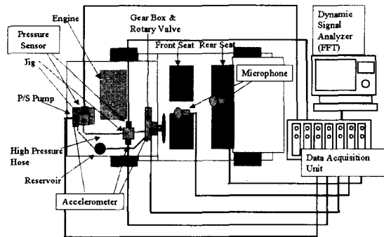
Fig. 2 Experimental set-up for NVH test
