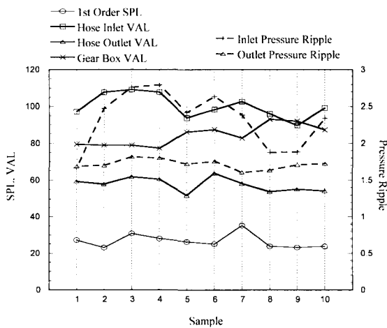
Fig. 9 The comparisons of 1 st order noise, vibration and pressure ripple between specimens
