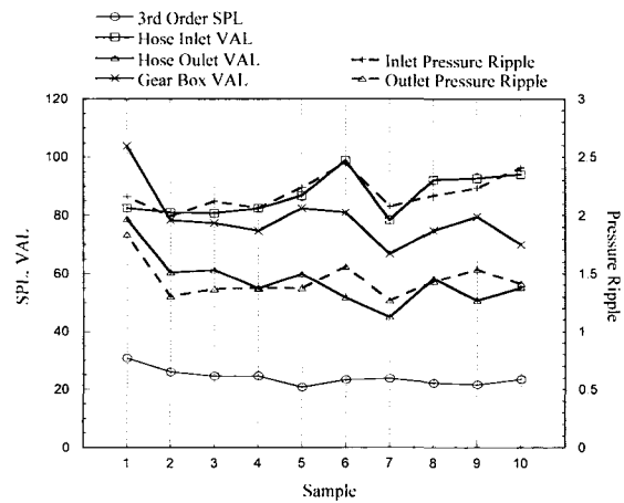
Fig. 11 The comparisons of 3 rd order noise, vibration and pressure ripple between specimens
