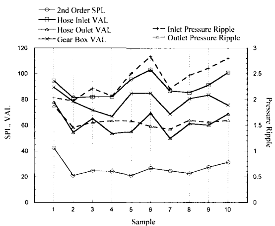
Fig. 10 The comparisons of 2 nd order noise, vibration and pressure ripple between specimens
