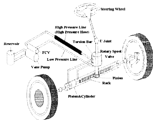
Fig. 1 A drawing of hydraulic power steering system
