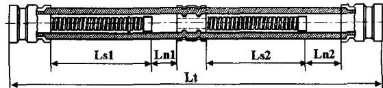
Fig. 3 High pressure hose for hydraulic power steering
