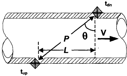
Fig. 1 Schematic diagram of transit time method
