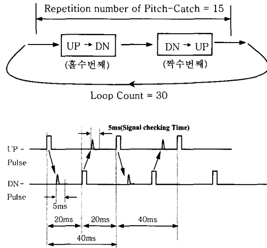
Fig. 4 Signal processing algorithm and ultrasonic trigger
