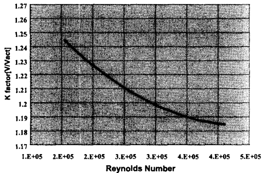
Fig. 7 Compensation factor of ultrasonic flowmeter
