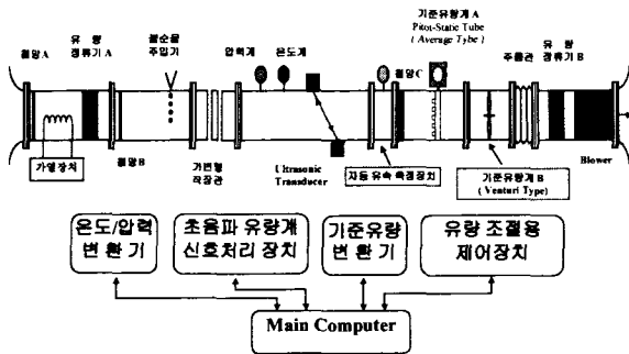
(b) Apparatus for the calibration of flowmeter
