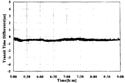
Fig. 6 Stability & repeatability test of flowmeter
