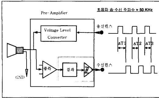
Fig. 3 Schematic diagram of pre - amplifier
