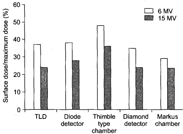
Fig. 5. Surface dose for 6 MV and 15 MV X-ray at 10×10 cm 2 , SSD=100 cm.
