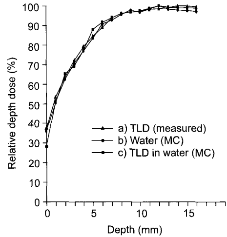
Fig. 4. Compared with Monte Carlo simulation and measured TLD data. a) measured data of TLD b) MC for pure water phantom and c) MC for imaginary TLD inserted in the water phantom surface.
