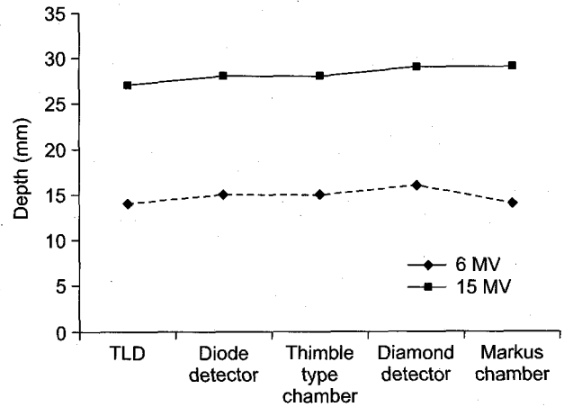
Fig. 6. Dose maximum depth for 6 MV and 15 MV X-ray at 10×10 cm 2 , SSD=100 cm.
