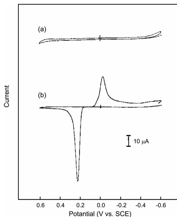
Figure 1. Cyclic voltammograms for the DPO-modified carbon paste electrode obtained (a) only in 0.1 M KNO 3 blank solution, (b) after dipping CPE in 1.0 \times 10^{-5} M Ag (I) solution for 10 min (deposition temp.: 25 °C, scan rate: 100 mV/s).
