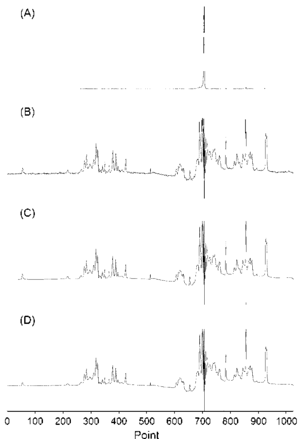
Figure 2. 1D ^1\text{H} -NMR spectrum obtained from a first FID of NOESY data of Zn-LHRH complex has an off resonance large water peak (A), and spectrum after application of a large solvent peak suppression by using SVD (B), and spectrum after application of noise suppression on the figure-(B) by using uniform threshold (C), and spectrum after treatment of universal threshold method (D).
