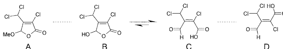
Figure 1. Various Forms of MX ( B, C, D ) and its analogue ( A )
