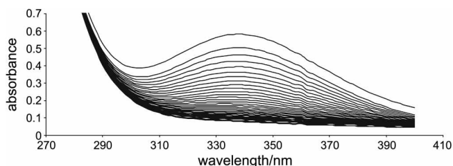
Figure 1. Repetitive scan for the decomposition of SNAP by aqueous sulfite at 15.0 °C. [\text{SNAP}] = 5 \times 10^{-4} \text{ mol dm}^{-3} , [\text{S}^{\text{IV}}]_{\text{T}} = 0.05 \text{ mol dm}^{-3} , I = 1.0 \text{ mol dm}^{-3} (NaCl), pH = 5.05 (buffer = Citric acid/ \text{HPO}_4^{2-} ), cycle time = 5 seconds.
