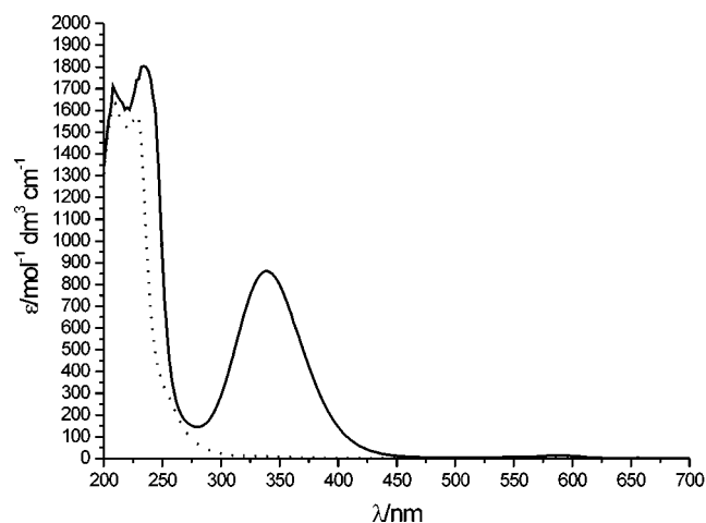
Figure 2. The spectral change in going from the reactant [SNAP with no aqueous sulfite] (—) to its decomposed products (....). [\text{SNAP}] = 1.51 \times 10^{-3} \text{ mol dm}^{-3} , [\text{S}^{\text{IV}}]_{\text{T}} = 0.02 \text{ mol dm}^{-3} , [\text{H}_2\text{EDTA}^{2-}] = 2 \times 10^{-3} \text{ mol dm}^{-3} , pH = 4.42. Buffer = citric acid/ \text{HPO}_4^{2-} .
