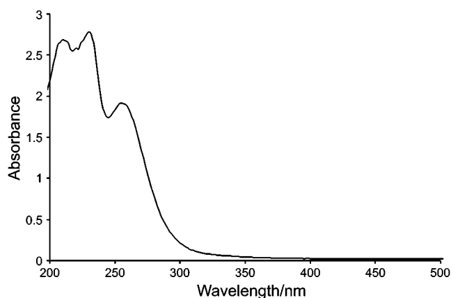
Figure 3. UV/Visible spectrum of the N-nitrosohydroxylamine-N-sulfonate ion at pH 4.51. [\text{SNAP}] = 5 \times 10^{-4} \text{ mol dm}^{-3} , [\text{S}^{\text{IV}}] = 0.10 \text{ mol dm}^{-3} , [\text{Na}_2\text{H}_2\text{EDTA}] = 1 \times 10^{-3} \text{ mol dm}^{-3} , I_{\text{Total}} = 1.0 \text{ mol dm}^{-3} (NaCl) at 20.0 °C.
