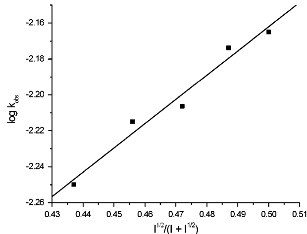
Figure 7. A plot of \log k_{\text{obs}} versus I^{1/2}/(1+I^{1/2}) for the decomposition of SNAP by aqueous sulfite at 30.0 °C.
