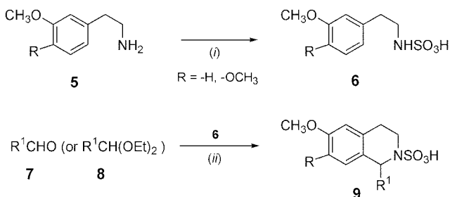
Scheme 1. Synthesis of 8 . Reagents and conditions: (i) 1) \text{ClSO}_3\text{H}\cdot\text{Et}_3\text{N} , -5\text{--}0^\circ\text{C} , 2) c\text{-HCl} ; (ii) \text{HCO}_2\text{H} .
