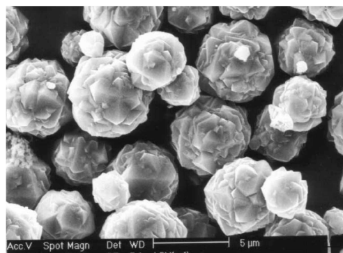
Figure 2. SEM image of as-synthesized LSX.
