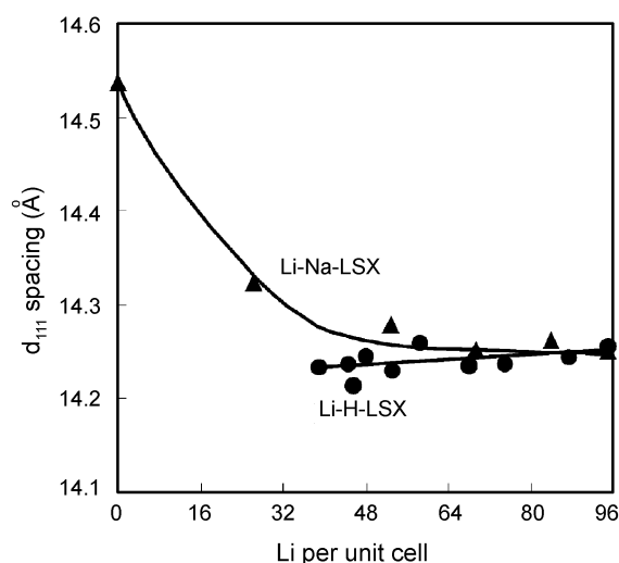
Figure 6. Change in d_{111} -spacing by Li content in Li-H-LSX (●) and Li-Na-LSX (▲).
