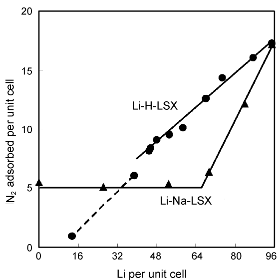
Figure 4. Change in the amount of nitrogen adsorbed by Li content in Li-H-LSX (●) and Li-Na-LSX (▲) at 760 torr, 20 °C.
