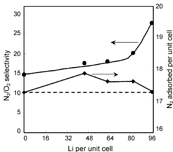
Figure 7. Effect of Li content on N_2/O_2 selectivity (●) and the amount of nitrogen adsorbed (▲) at 20 °C, 760 torr in Li-Ca-LSX.
