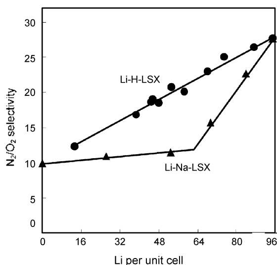
Figure 5. Change in N_2/O_2 selectivity by Li content in Li-H-LSX (●) and Li-Na-LSX (▲) at 20 °C. The selectivity was calculated by N_2 adsorbed at 608 torr and O_2 adsorbed at 152 torr.
