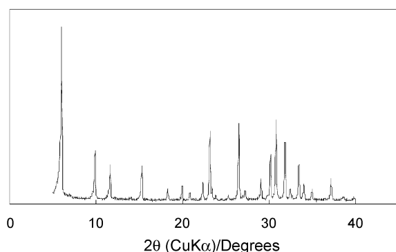
Figure 1. XRD pattern of as-synthesized LSX.
