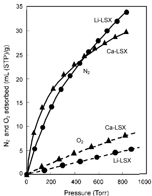
Figure 3. N_2 (solid line) and O_2 (broken line) adsorption isotherms of Li-LSX (●) and Ca-LSX (▲) at 20 °C.
