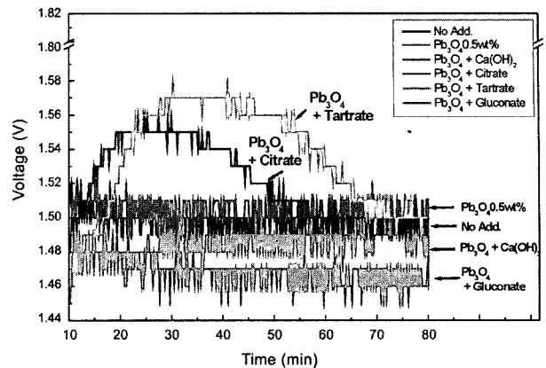
Fig. 6. Variation of discharge voltage of the 1st cycle with discharging current 5 A for 70 min.
