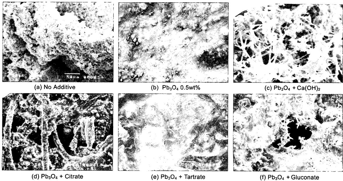
Fig. 10. SEM photographs of Zn specimen in KOH 40 wt% with additives after 3days submerged.
