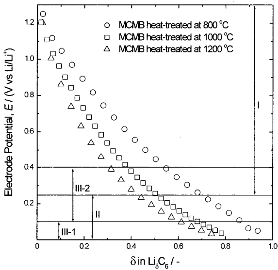
Fig. 11. The galvanostatic intermittent discharge (electrode potential) curve measured on the PVDF-bonded MCMB800(○), MCMB1000(□) and MCMB1200(Δ) composite electrodes in 1 M LiPF 6 -EC/DEC solution. Region I, II, III-1 and III-2 represent the potential ranges necessary for lithium deintercalation from the sites for Type I, Type II, Type III-1 and Type III-2, respectively.
