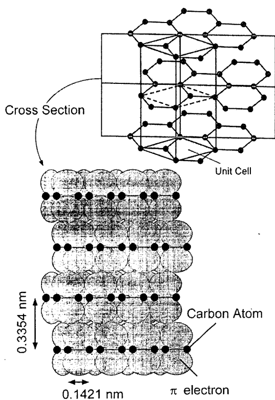
Fig. 1. Structure of hexagonal graphite showing ABAB stacking, and schematic diagram of cross-section of stacking layers considering the thickness of each carbon layer.
