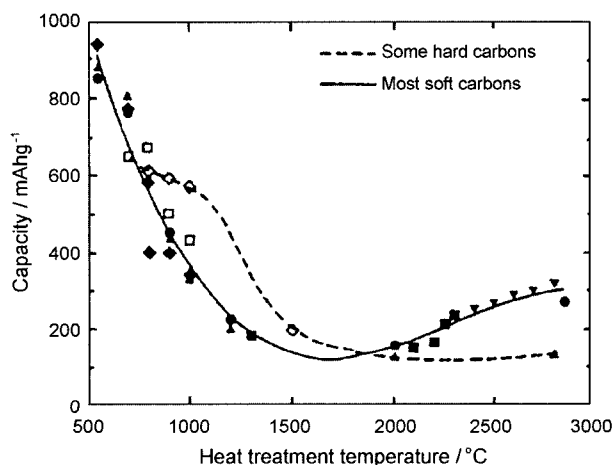
Fig. 5. Relationship between reversible specific capacity and heat-treatment temperature of various soft carbons and hard carbons 15) .
