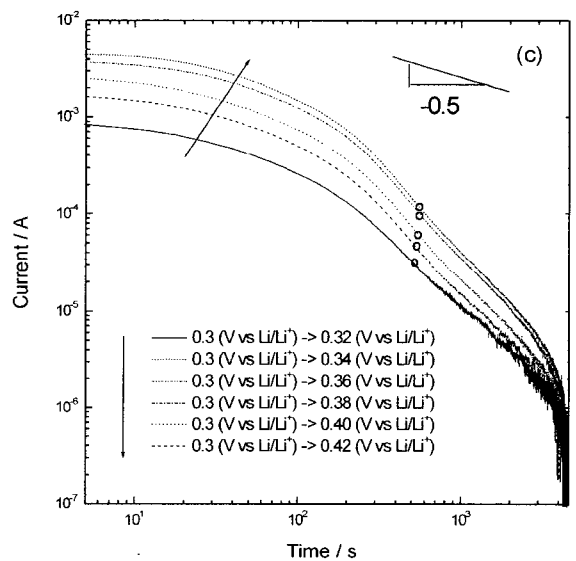
Fig. 12. The anodic current transient experimentally obtained from the PVDF-bonded MCMB800 composite electrode in 1 M LiPF 6 -EC/DEC solution at the potential jumps of E = (a) 0.05 V Li/Li + , (b) 0.20 V Li/Li + and (c) 0.30 V Li/Li + to various lithium extraction potentials E_{ext} as indicated in figure. Symbols □ and ○ denote inflexion points.
