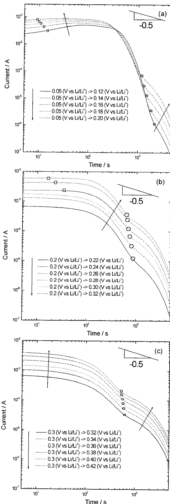
Fig. 13. The anodic current transient theoretically calculated based upon the modified McNabb-Foster equation at the potential jumps of E = (a) 0.05 V Li/Li + and (c) 0.30 V Li/Li + to various lithium extraction potentials E_{ext} under the 'cell-impedance-controlled' constraint, by taking A_{ea} = 1.56 \text{ cm}^2 , \bar{D}_{Li} = 2 \times 10^{-10} \text{ cm}^2 \text{ s}^{-1} , R_{cell} = 27.8 \ \Omega and R^* = 5 \ \mu\text{m} . Symbols □ and ○ denote inflexion points.
