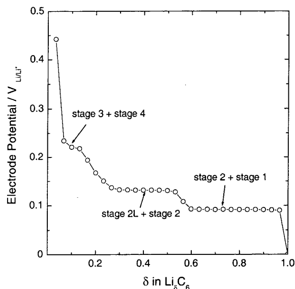
Fig. 7. The galvanostatic intermittent discharge curve obtained from the SFG6 graphite composite electrode in a 1 M LiPF 6 -EC/DEC solution.
