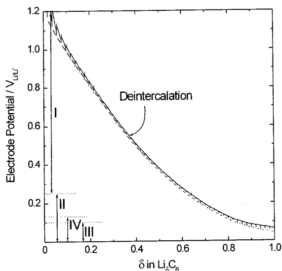
Fig. 14. The galvanostatic intermittent discharge curve measured on the Carbotron-P hard carbon composite electrode in a 1 M LiPF 6 -EC/DEC solution. Region I, II, III and IV represent the potential ranges necessary for lithium deintercalation from the sites for Type I, Type II, Type III and Type IV, respectively.
