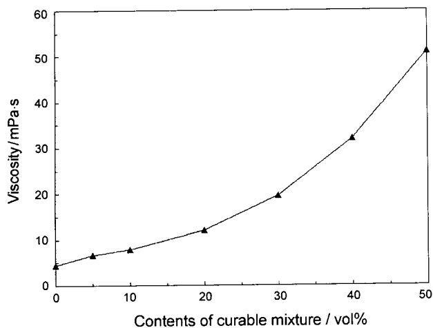
Fig. 3. Relationship between the viscosity of the precursor and the contents of the curable mixture.
