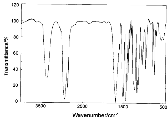
Fig. 2. FTIR spectrum of polyurethane acrylate oligomer.
