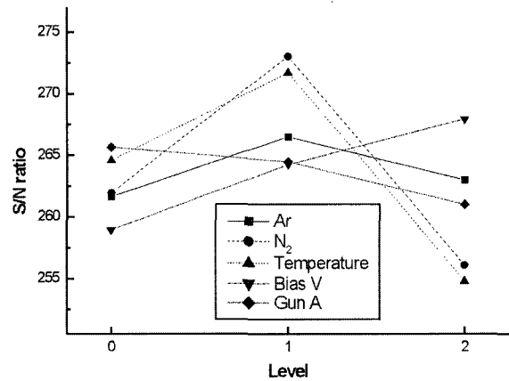
Fig. 3. S/N Ratio of Total Experiment Factor
