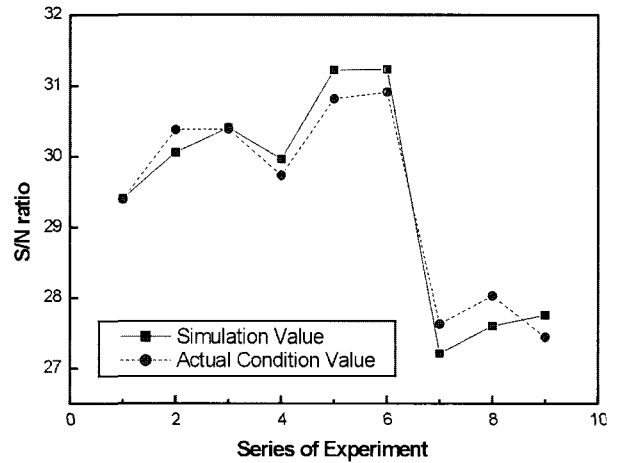
Fig. 4. Comparison Between Neural Network and Experimental Value
