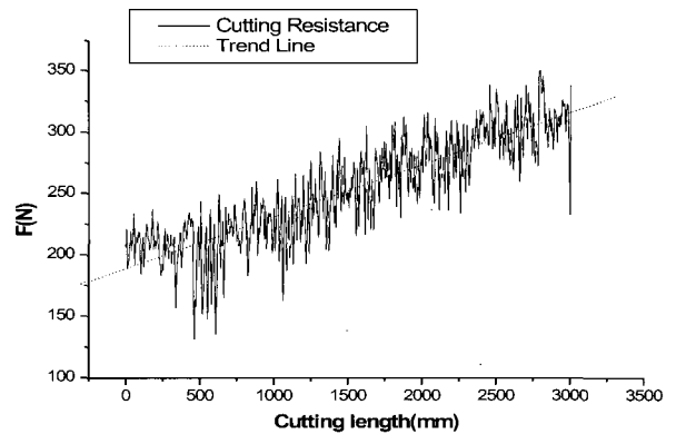
Fig. 1. Gradient of Cutting Force
