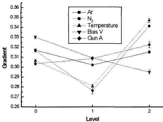
Fig. 2. Gradient Variation of Total Experimental Factor.
