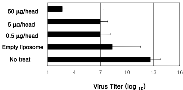
Figure 1. Three weeks after immunization with XEPs-liposome or empty liposome as control, mice were challenged with 1×10 7 pfu/head of rVV-HBx i.p.. The ovaries were harvested and the viral titer was measured using TK 143B cells. The mean viral titre±S.E. value of three or four mice in each group is shown.
