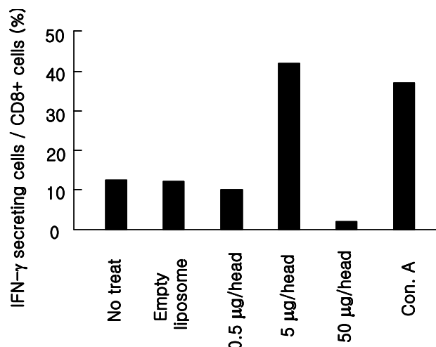
Figure 3. Three weeks after immunization with XEPs-liposome, or empty liposome as control, mice were challenged with 1 \times 10^7 pfu/head of rVV-HBx i.p. Five days after challenge, the spleens were harvested and restimulated with either the appropriate peptide (20μg/ml) on APCs, Con. A (2μg/ml, positive control), or vehicle (negative control) for 5hrs in media supplemented with GolgiStop. Cells were stained with FITC-conjugated anti-CD8 (PharMingen), washed, fixed, and permeabilized with Perm Wash/Fix (PharMingen) and further stained with PE-conjugated anti IFN-γ.
