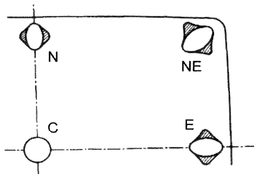
Fig. 3. Astigmatism of an electron beam generated by an electron gun with rotational symmetry and deflected with the most uniform field, at the right top quadrant of the screen. The shaded areas indicate haze.
