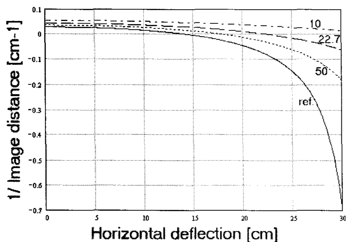
Fig. 7. The required vertical reciprocal image distance of the gun as a function of deflection, for various focal lengths (indicated in cm in the figure) of the fixed quadrupole.
