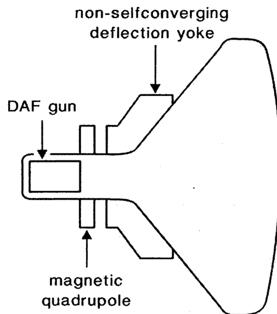
Fig. 5. Basic elements of the DAF-Q system; a DAF gun, a quadrupole driven with a line deflection dependent current and a deflection yoke that is only self convergent in combination with the driven magnetic quadrupole.
