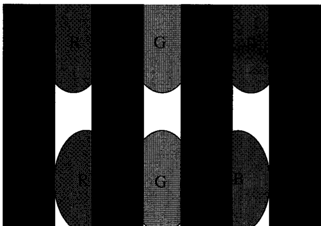
Fig. 9. Microscopic spots at low (top) and high (below) beam currents behind the black matrix lines on the screen. Due to space charge repulsion the microscopic spots of one triplet creep closer to each other.
