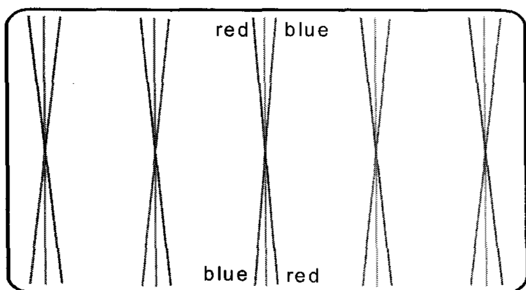
Fig. 2. This convergence error pattern arises from a vertical CRT alignment error, but it can be corrected relatively easily by means of a quadrupole.
