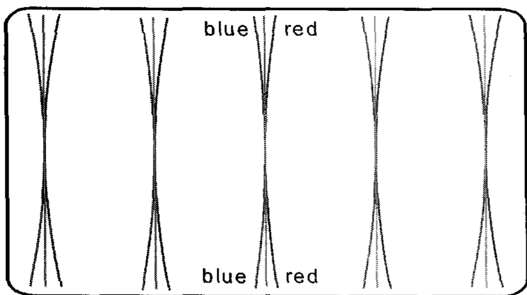
Fig. 1. This convergence error pattern is sometimes the best obtainable result due to an improper length of the deflection fields, but it can be eliminated by means of a quadrupole.
