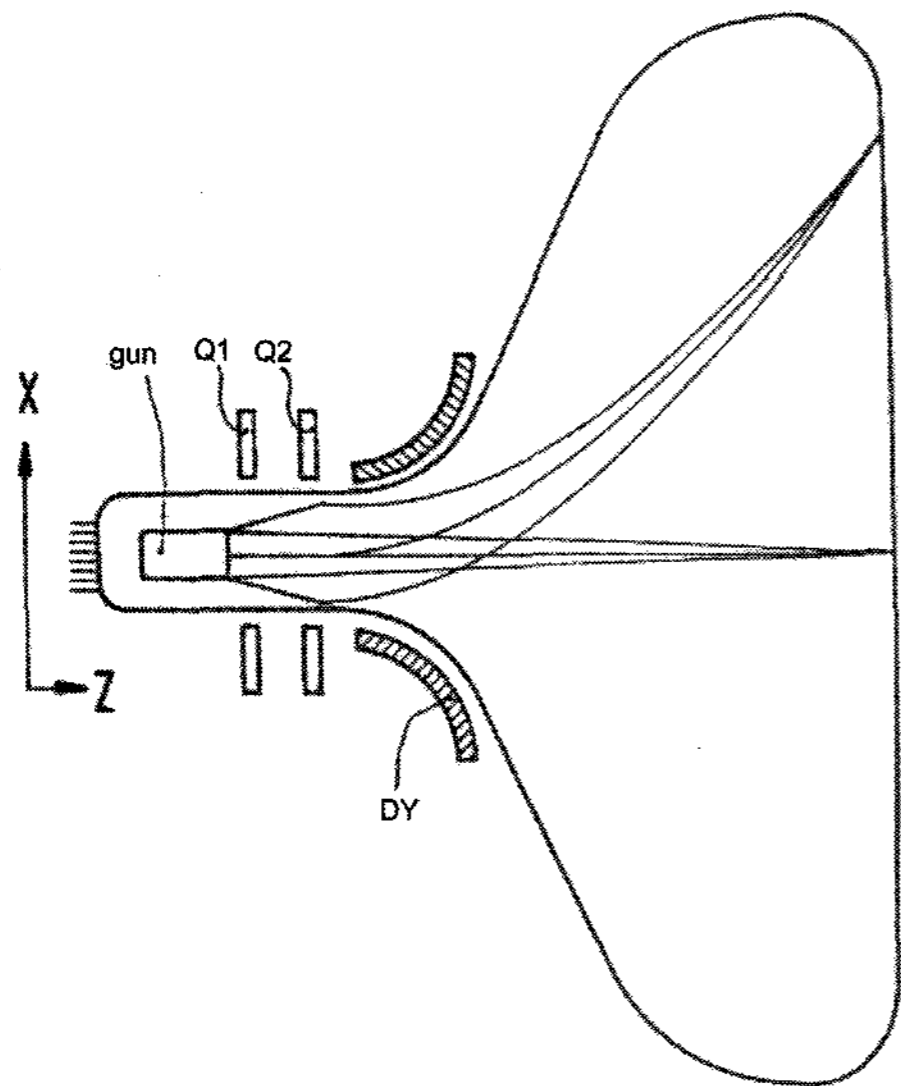
Fig. 6. Basic elements of the DAF- Q^2 system, a DAF gun, two quadrupoles and a fully self-converging deflection yoke.
