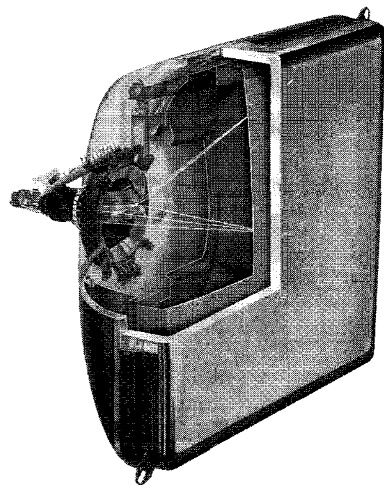
Fig. 8. A Real Flat tube in which the shadow-mask is made more curved in the vertical direction than the inner surface of the screen. This is possible because two quadrupoles are used to reduce the (virtual) pitch of the gun.
