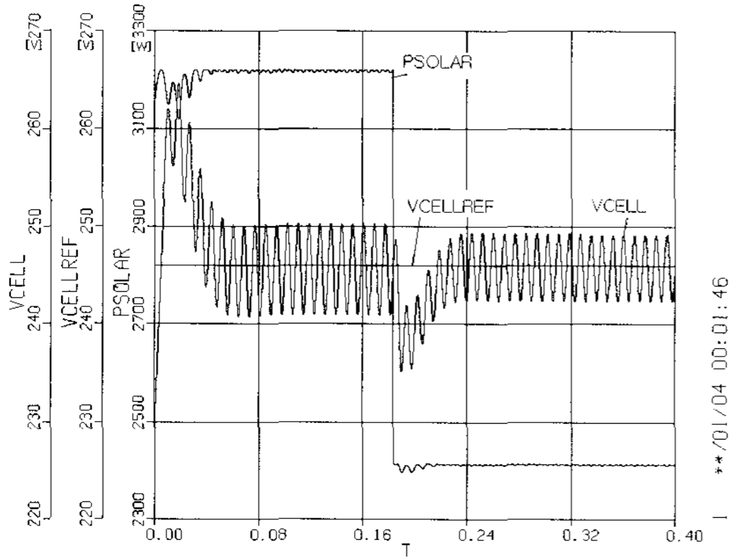
그림 13. Simulation results of constant voltage MPPT control in the utility interactive inverter.
