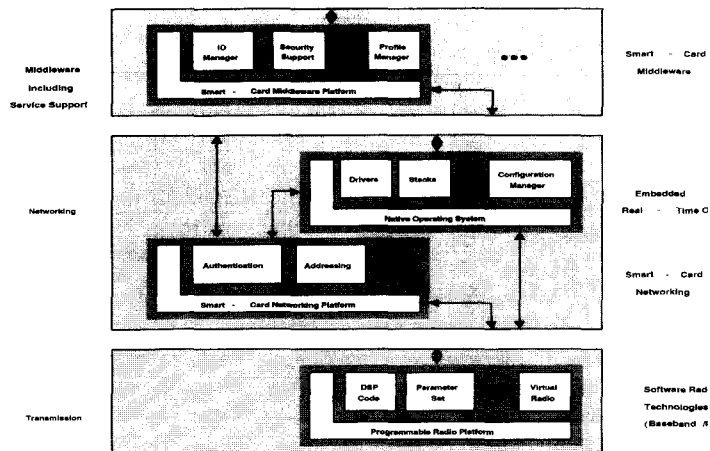
Fig. 6. Mobile device architecture.
