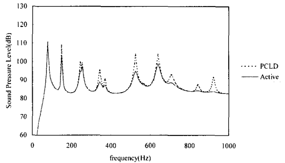
Fig. 5 Controlled sound power radiation from a simply supported [45/45/0/90]s composite plate (with 3 PZT S/As and VE)
