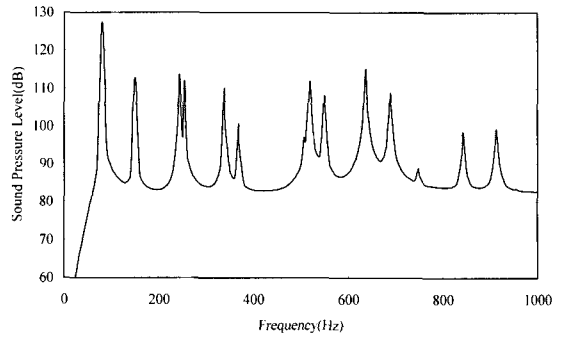
Fig. 4 Sound power radiation from a simply supported [45/45/0/90]s composite plate (with 3 PZT S/As)
