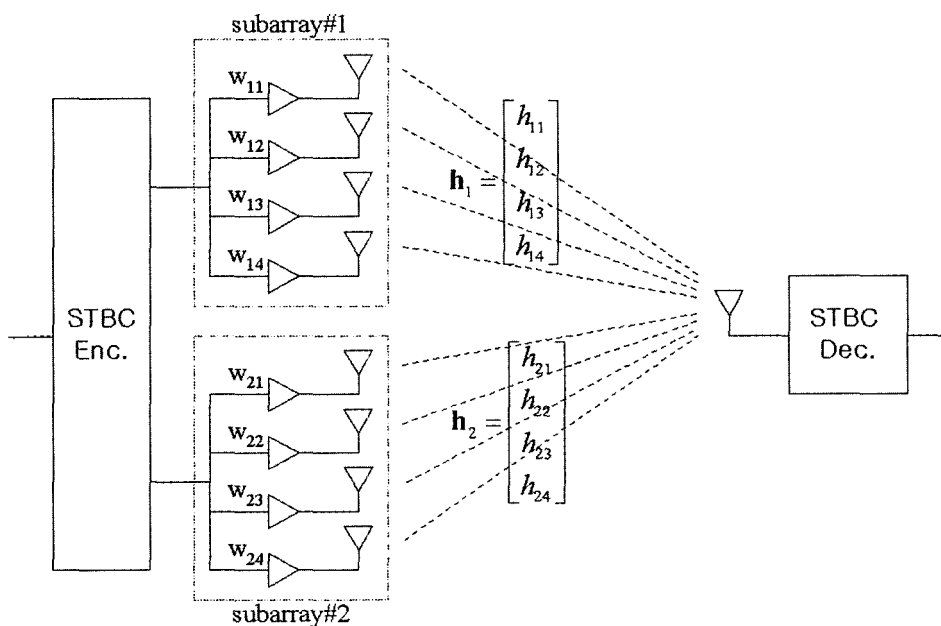
Figure 1. Model of the proposed TEBS system.
