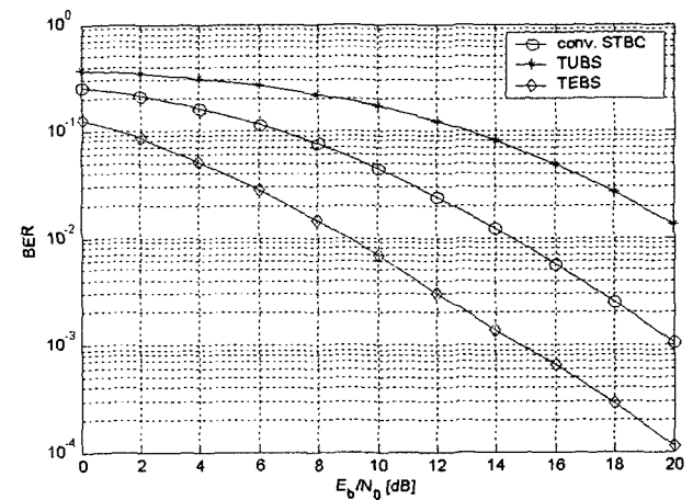
Figure 4. Spatially heavily correlated channel.
