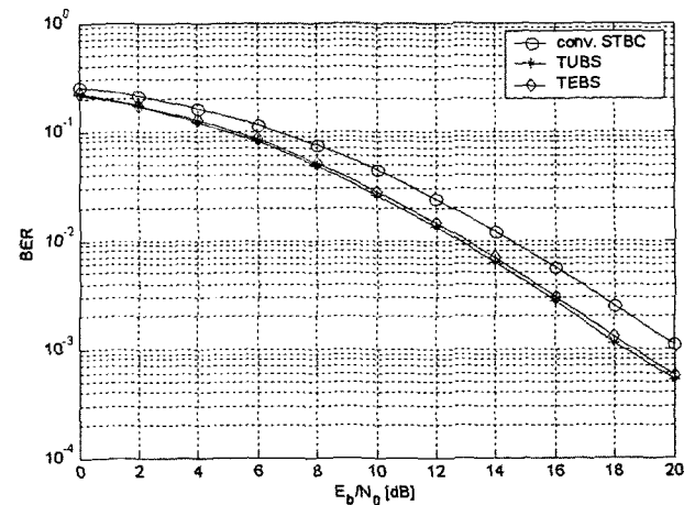
Figure 3. Spatially weakly correlated channel.
