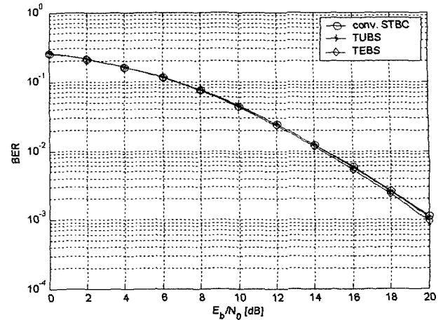
Figure 2. Spatially uncorrelated channel.
