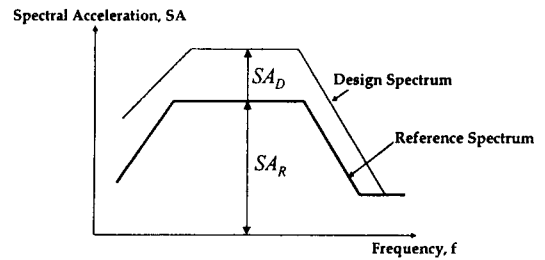
Fig. 1. Spectral Accelerations for Spectrum Shape Factor, F_{ss}
