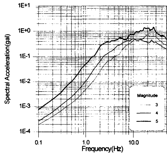
Fig. 6. Mean Response Spectra for Earthquake
