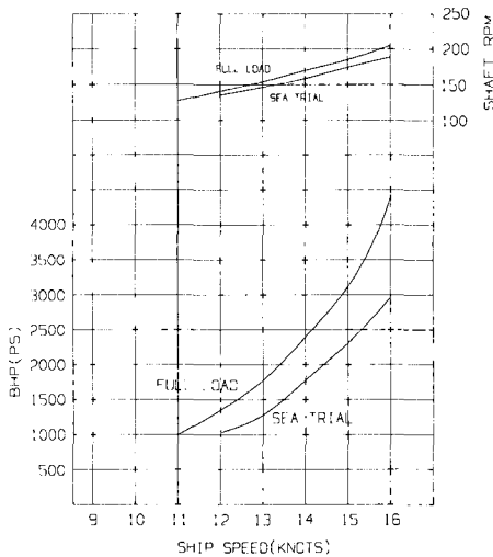
Fig. 11 Speed-horse power curve on design ship
