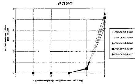
Fig. 4 Irregular response of deck wetness at F.P
