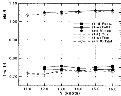
Fig. 10 Comparison of self-propulsion coefficient
