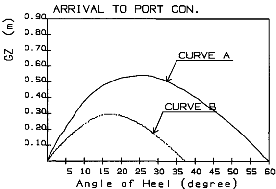
Fig. 3 Curve of the GZ on arrival to port condition.
