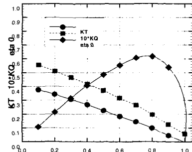
Fig. 9 Open-water characteristics of the stock propeller
