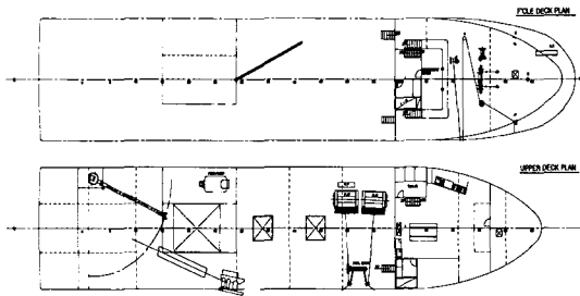
Fig. 1 Initial deck arrangement of 2 vessel purse seiner
