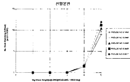
Fig. 5 Irregular response of slamming at ST. 17
