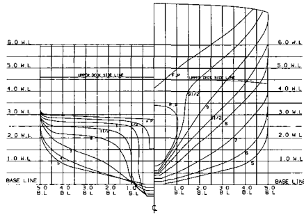
Fig. 2 Body plan of design ship
