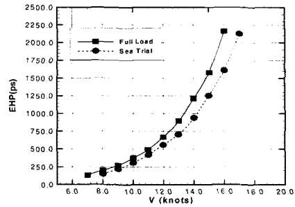
Fig. 8 Comparison of effectiveness horsepower
