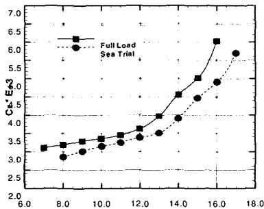
Fig. 7 Comparison of Residual resistance coefficient
