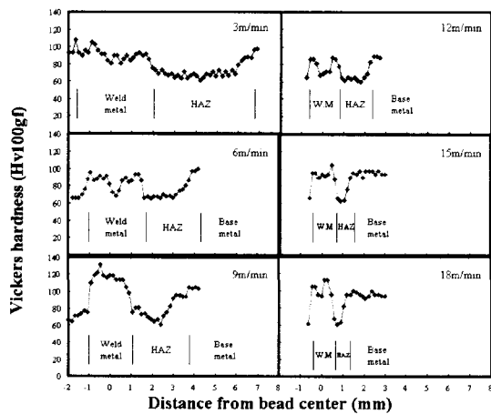
Fig. 6 Hardness distribution in the laser welded joint of A6N01 alloy with Ni 5wt%-Zr3wt% in Al-12Si filler metal at different travel speeds
