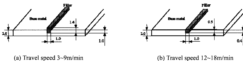
Fig. 1 Setup of filler metals on base metal
