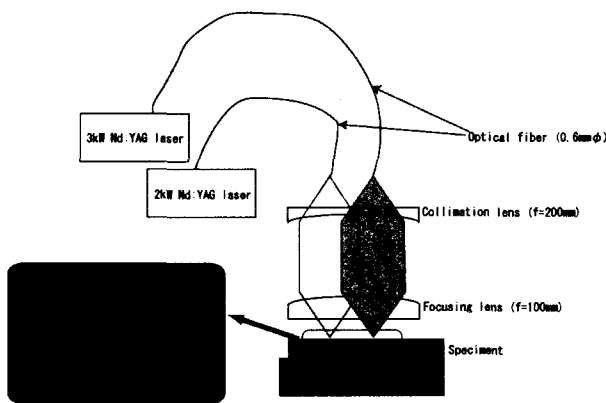
Fig. 2 Schematic of twin beam Nd:YAG laser
