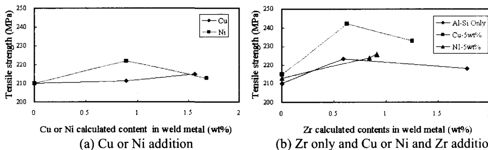
Fig. 10 Effect of alloying content in A6N01 weld metal on tensile strength after laser welding at 9m/min
