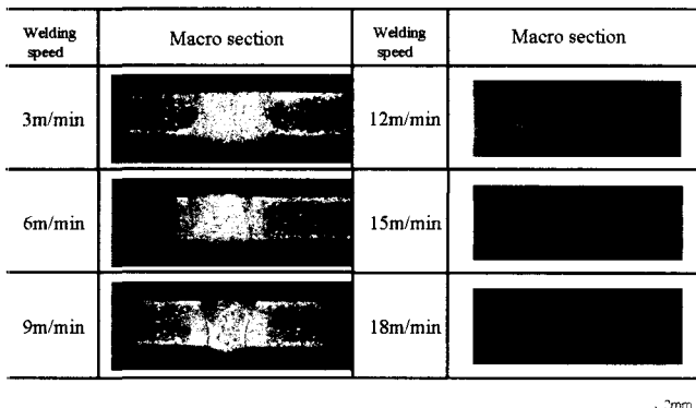
Fig. 5 Cross section of laser weld of A6N01 alloy with Al-12Si base filler metal
