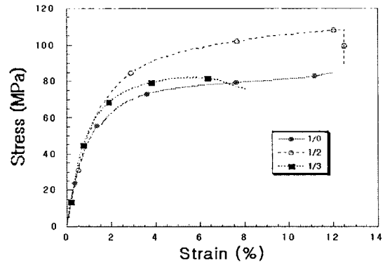
Fig. 9 Shear stress-strain response for twisted glass/epoxy specimens.
