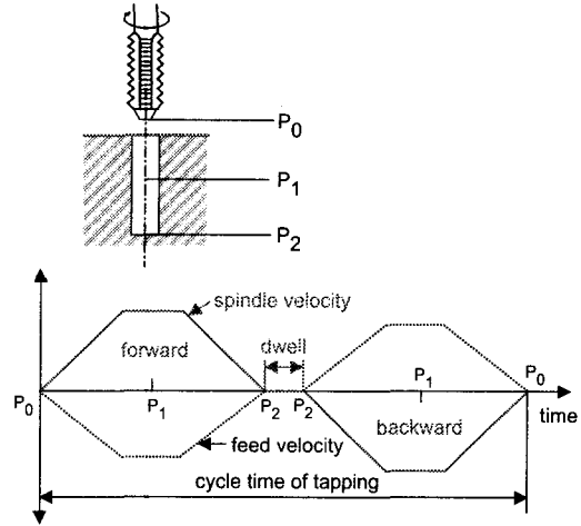
Fig. 2 Tapping cycle for time variant
