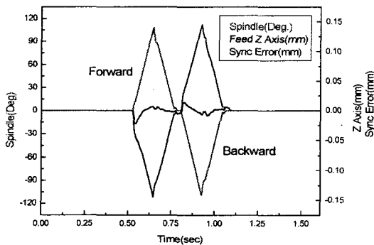
Fig. 9 Diagram of synchronizing error for M3 and depth 2 times diameter tapping
