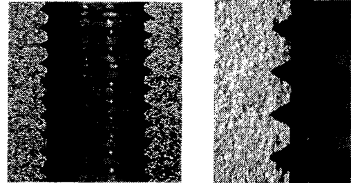
Fig. 10 Cross section for machined female screw for 10,000rpm tapping
