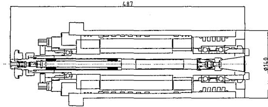
Fig. 5 Structure for tapping machine spindle
