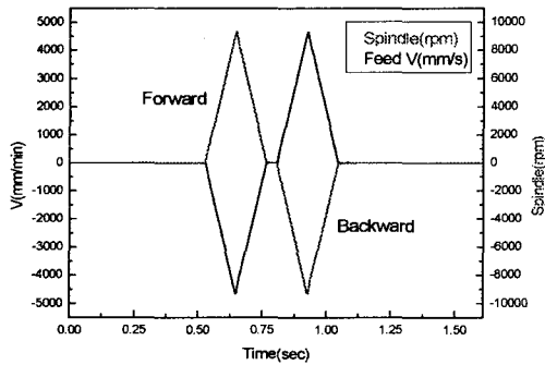
Fig. 8 Diagram between spindle speed and feeding motor for M3 and depth 2 times diameter tapping
