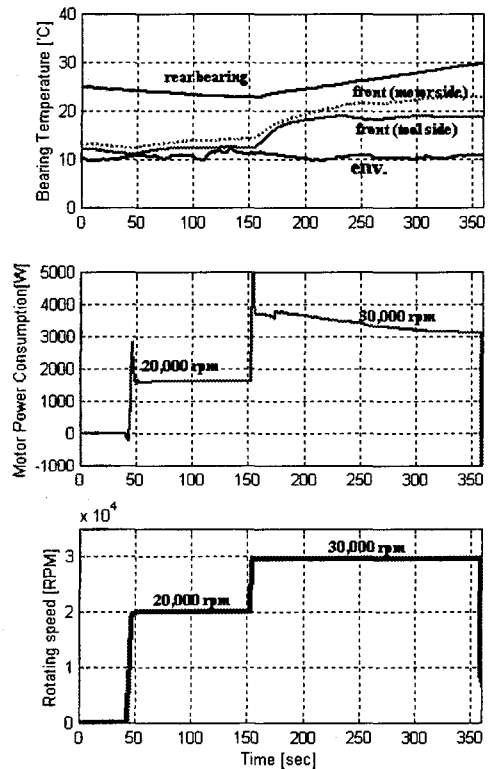
Fig. 6 Power consumption and temperature variation for spindle
