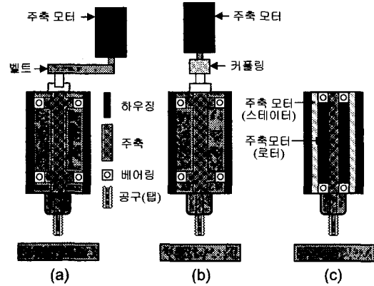
Fig. 1 Spindle structures for tapping machine (a) Belt drive type, (b) Direct drive type, (c) Built-In type
