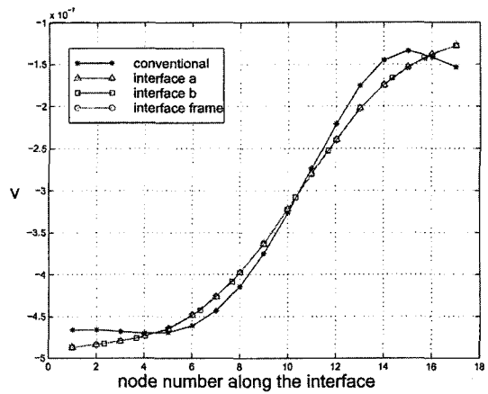
Fig. 15 Vertical displacement v along the interface ( k/E=10^4 )
