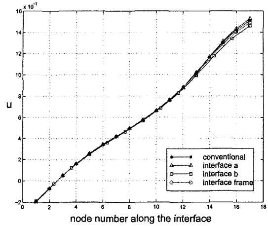
Fig. 8 Horizontal displacement u along the interface ( k/E=10^1 )
