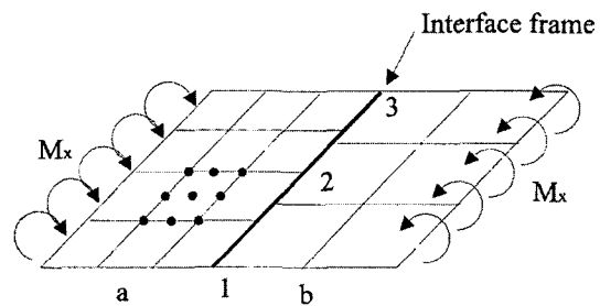
Fig. 17 Plate under pure bending
