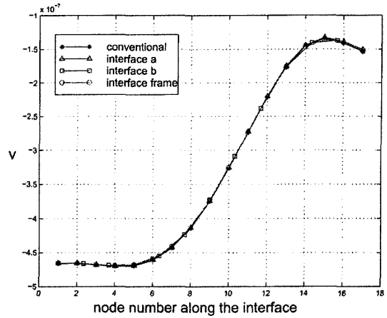
Fig. 13 Vertical displacement v along the interface ( k/E=10^2 )
