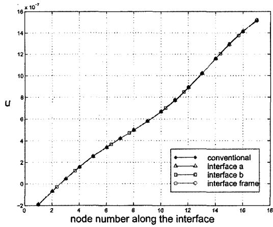
Fig. 10 Horizontal displacement u along the interface ( k/E=10^3 )
