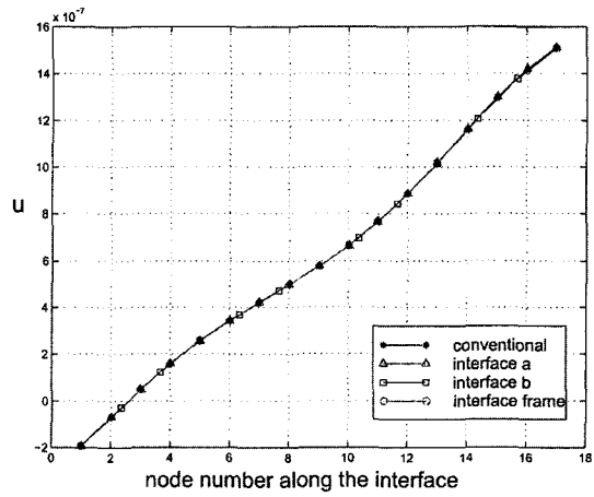
Fig. 9 Horizontal displacement u along the interface ( k/E=10^2 )
