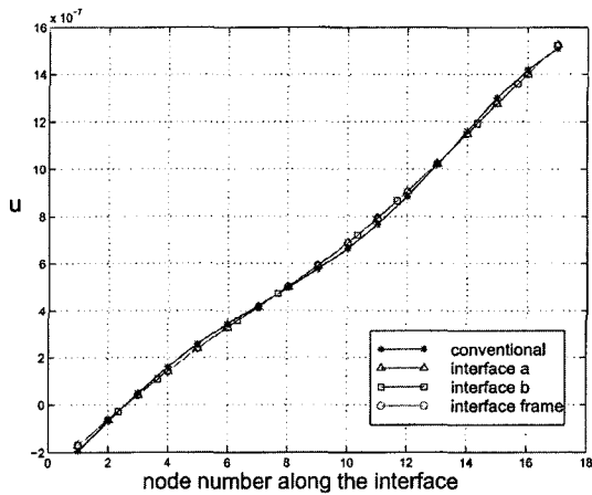
Fig. 11 Horizontal displacement u along the interface ( k/E=10^4 )
