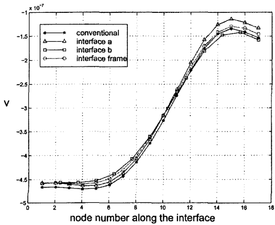
Fig. 12 Vertical displacement v along the interface ( k/E=10^1 )
