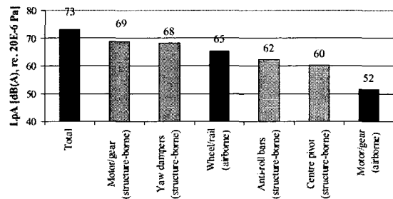
Fig. 8 Comparison of noise source for section 7 above the compartment motorized car while driving at 300 km/h in free field (HVAC and pressurization unit noise is not included)
