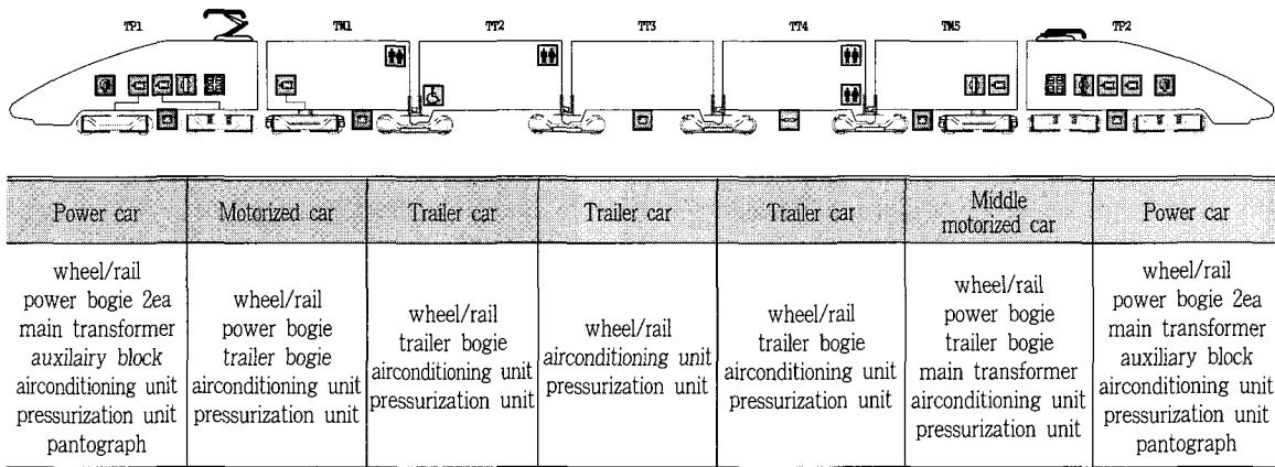
Fig. 1 Formation of KHST7 and main noise sources
