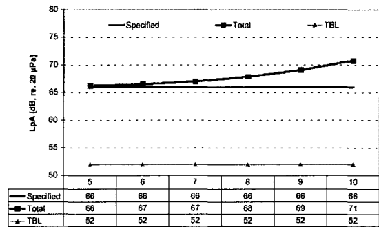
Fig. 3 Noise distribution in trailer car compartment during free-field driving at 300 km/h (HVAC and pressurization unit noise is not included)
