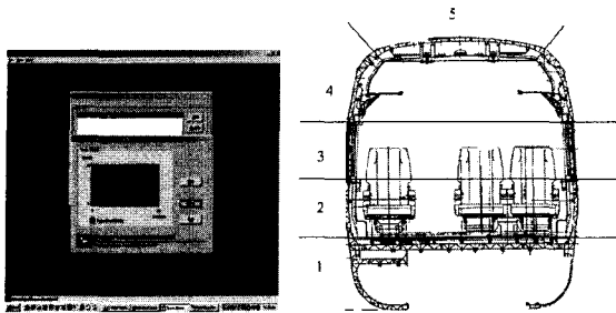
Fig. 2 Analysis program (TRAINNOISE) and example of noise prediction model (trailer car: section view)
