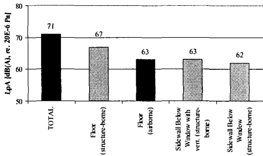
Fig. 4 Comparison of transmission path for section 10 above the compartment trailer car while driving at 300 km/h in free field(HVAC and pressurization unit noise is not included)
