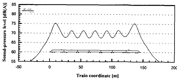
Fig. 11 Predicted A-weighted sound-pressure level from stationary car(current design)
