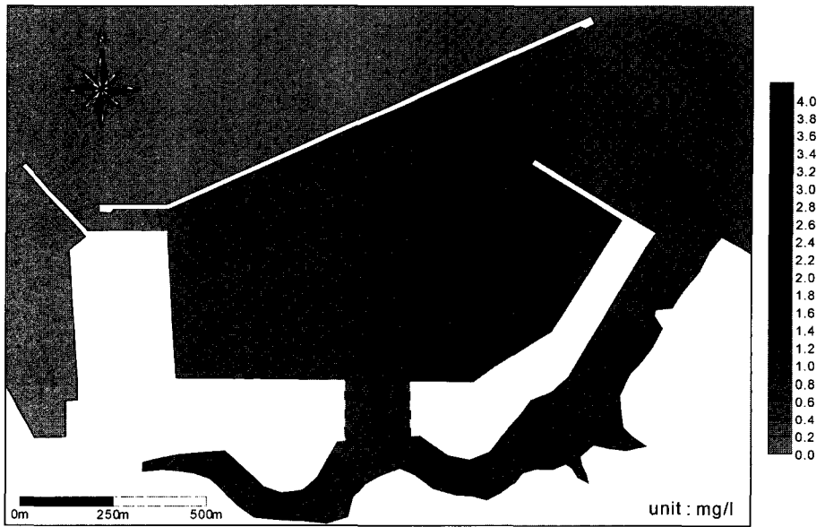
Fig. 19. Concentration distribution for instantaneous discharge with levee(after 7 days).
