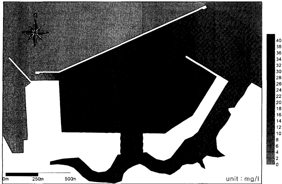
Fig. 15. Concentration distribution for continuous contaminant source with levee(after 30 days).
