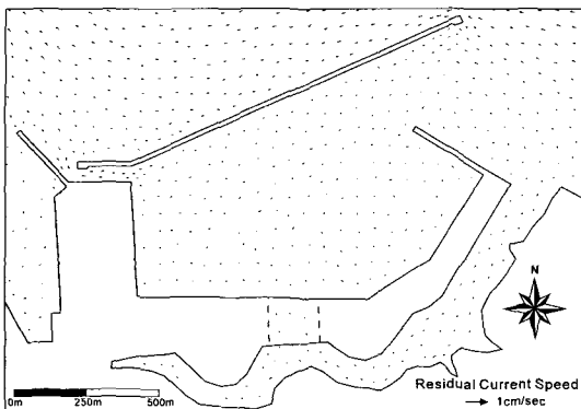
Fig. 12. Residual current distribution with flow channel.
