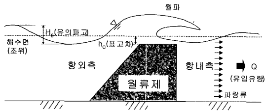
Fig. 1. Conceptual diagram of water influx by overflow levee.
