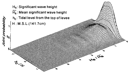
Fig. 8. Joint probability of significant wave height and tidal level.
