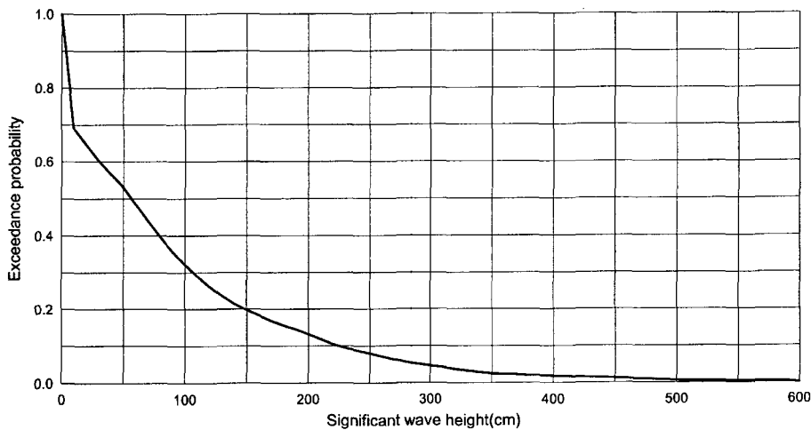
Fig. 7. Exceedance probability of wave height at site of levee proposed.
