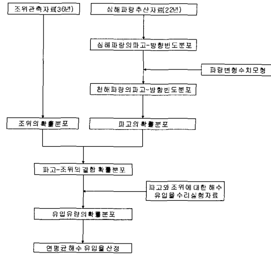
Fig. 3. Flow diagram for the calculation of annual mean water discharge through overflow levee.
