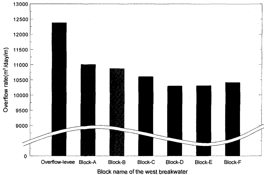
Fig. 10. Variation of annual influx according to levee sites.
