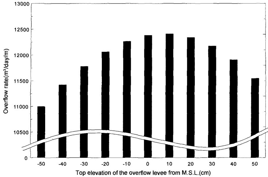
Fig. 11. Variation of annual influx according to top level of the levee.
