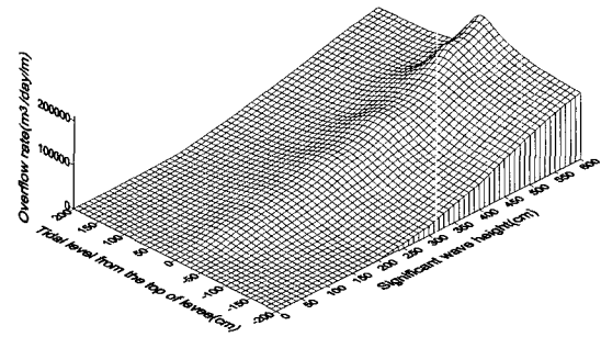
Fig. 5. Perspective view of water influx through levee.
