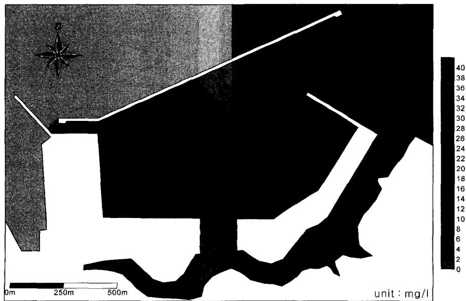
Fig. 14. Concentration distribution for continuous contaminant source with flow channel(after 30 days).
