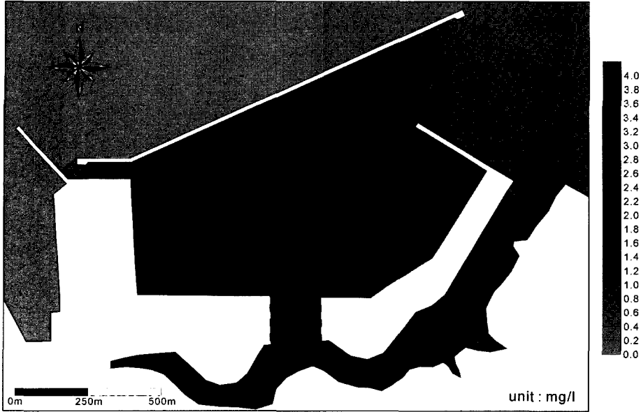
Fig. 18. Concentration distribution for instantaneous discharge with flow channel(after 7 days).
