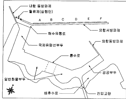
Fig. 2. Lay-out of Jeju outer port.
