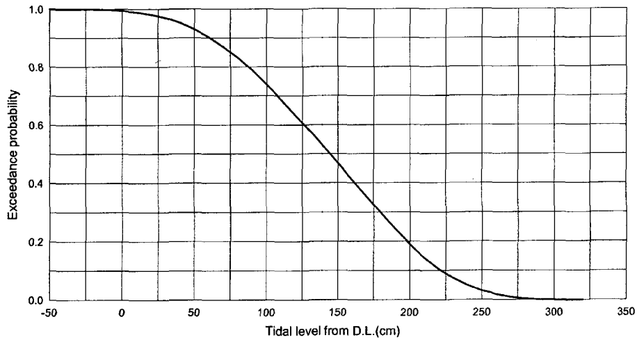
Fig. 6. Exceedance probability of water level at Jeju port.
