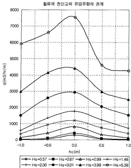
Fig. 4. Variation of influx according to significant wave heights and top level of the levee.
