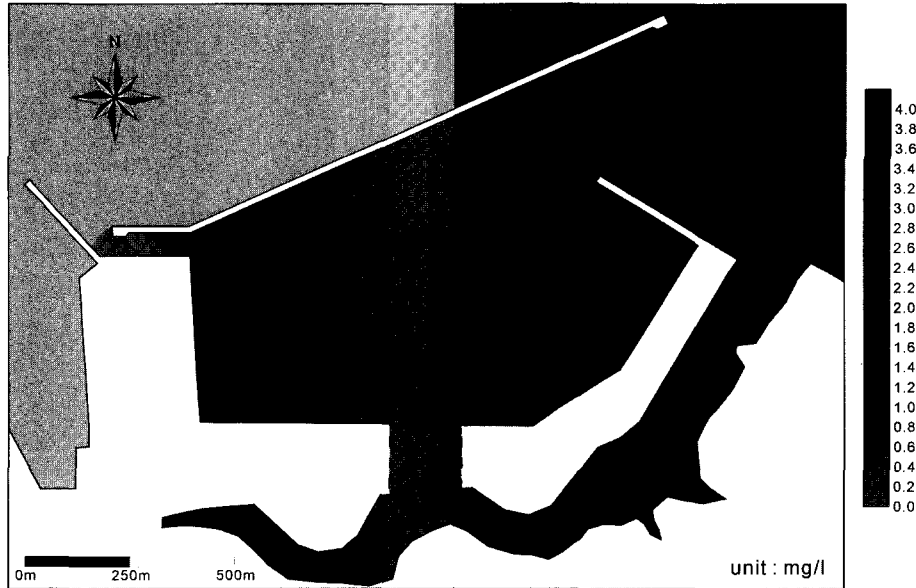
Fig. 16. Concentration distribution for instantaneous discharge with flow channel(after 3 days).
