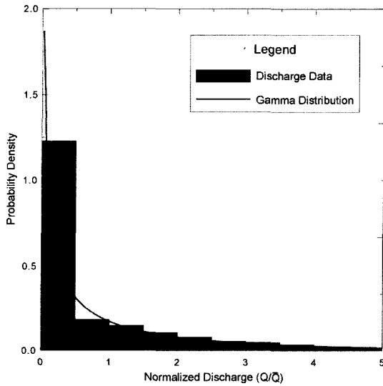
Fig. 9. Histogram of discharge through levee and corresponding Gamma distribution.
