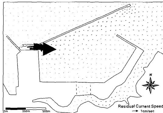
Fig. 13. Residual current distribution with overflow levee.
