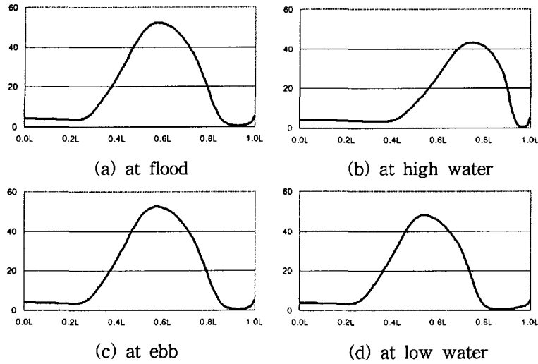
Fig. 2. Transitions of turbidity maximum at the Youngsan River estuary.
