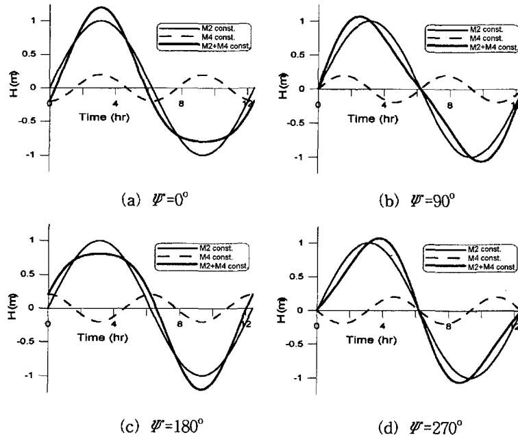
Fig. 1. Tidal distortions corresponding to the relative phases.
