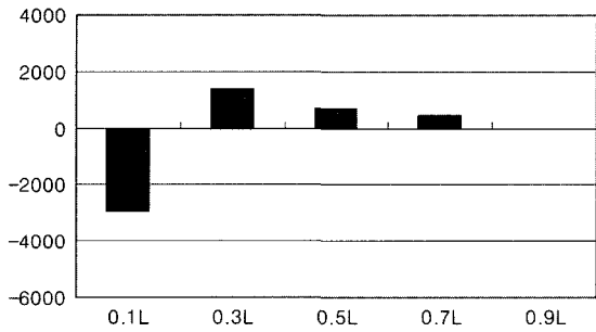
Fig. 3. Suspended sediment flux(g/m 2 )(Keum River estuary).
