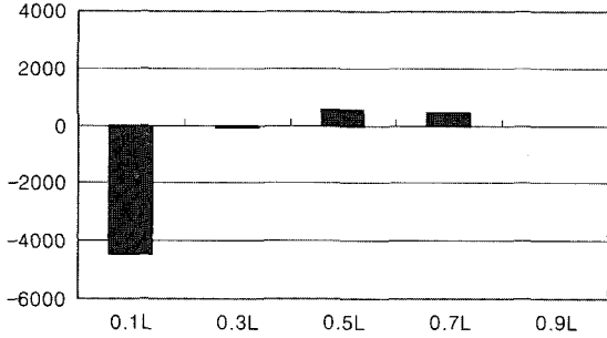
Fig. 6. Suspended sediment flux(g/m 2 )(Keum River estuary; low tide dominance).
