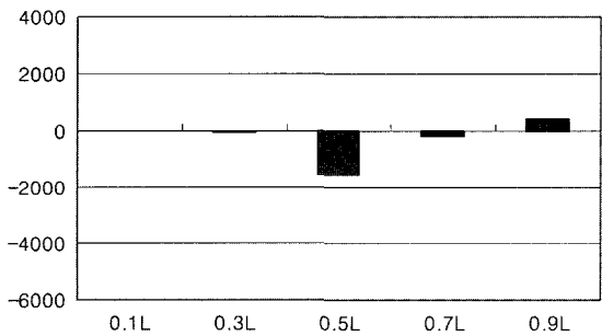
Fig. 4. Suspended sediment flux(g/m 2 )(Youngsan River estuary).
