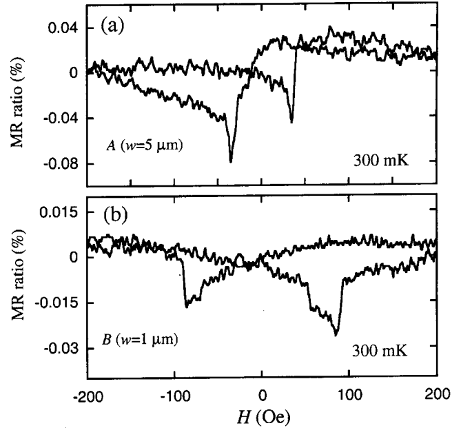
Fig. 5. Variation in the anisotropic magnetoresistance of (a) permalloy contact A and (b) contact B , respectively, when a magnetic field is swept up along the long axis of the contacts.
