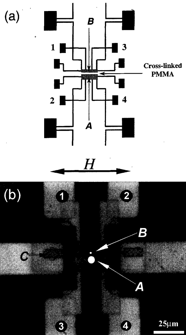
Fig. 2. (a) Schematic diagram of the device and (b) optical micrograph showing permalloy contacts A and B . The connections between the contacts A and B with the extended NiCr/Au are also shown. C indicates a contact pad, which is a part of the structures connecting with NiCr/Au contacts for MR measurements. The dots on the center of the contacts denote approximate laser beam spot size for MOKE measurements.
