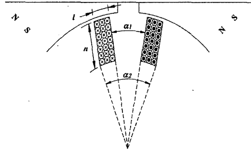
Fig. 4 Configuration of coil topology
