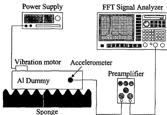
Fig. 9 Test setup for acceleration measurements
