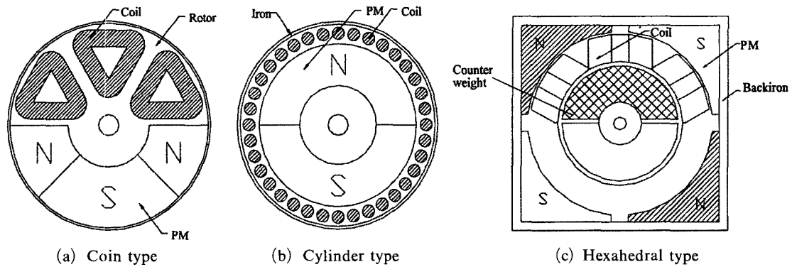
Fig. 1 Schematics of various vibration motors
