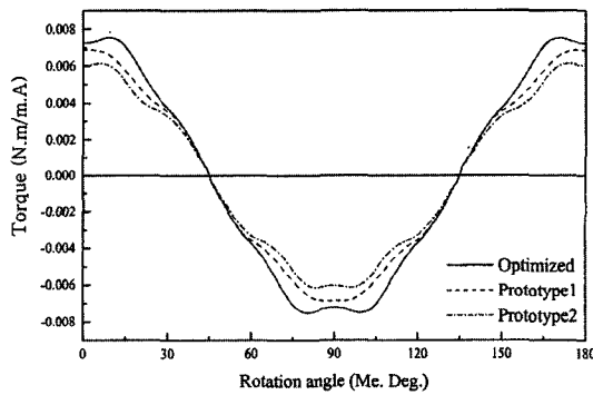
Fig. 7 Comparison of output torque between prototypes and optimized model
