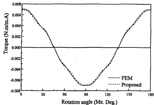
Fig. 5 Torque waveform by single coil with unit current input
