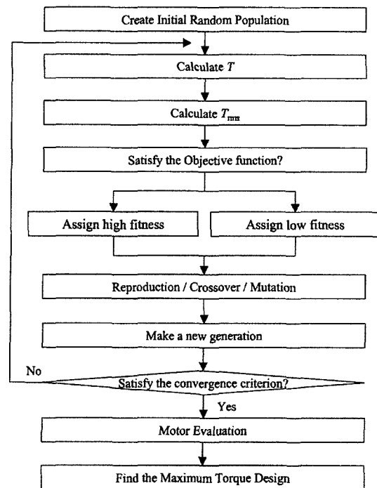
Fig. 6 Flow chart of genetic algorithm
