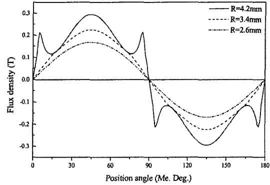
Fig. 3 Flux density distribution calculated by FEM
