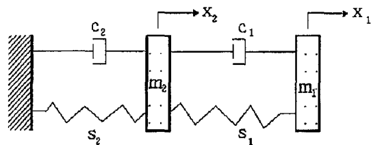
Fig. 1 Coupled Duffing's oscillator
