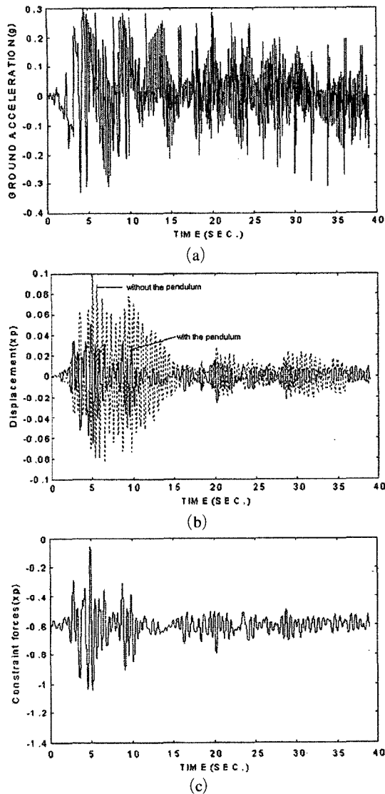
Fig. 4 Dynamic responses with or without the pendulum ; (a) North-south components of El-Centro earthquake in 1940, (b) displacement responses with or without the pendulum, (c) constraint forces acting in the x_p direction
