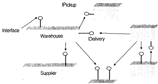
Focus on behavior: stored data, implemented procedures, other interfaces remain completely hidden
