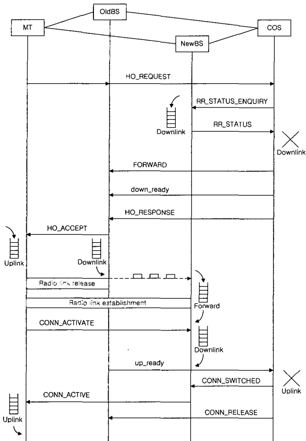
(Figure 3) Signaling message flow of handoff process
