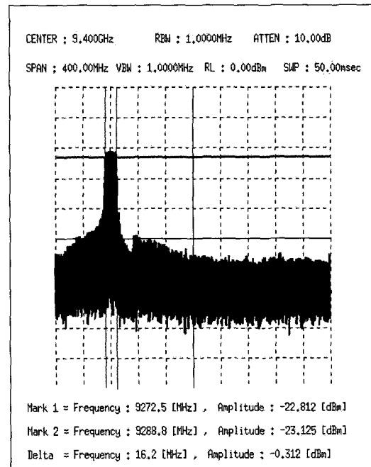
(a) 잡음대역폭(=16MHz)
