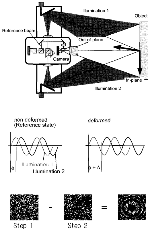
Fig. 1 Principle of 3D-ESPI System, wave profile and Speckle Pattern Images
