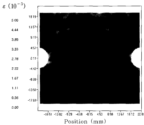
Fig. 5 Strain distribution of Type II under 150kN
