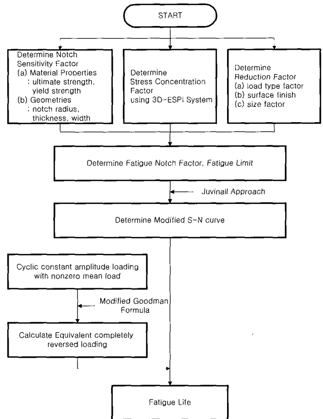
Fig. 7 Stepwise procedure for fatigue life calculation
