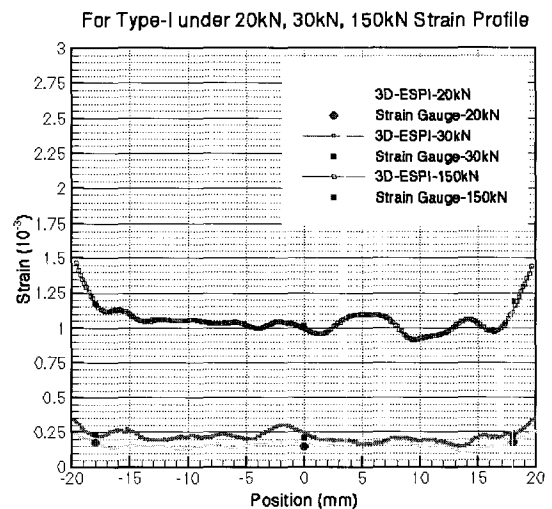
Fig. 4 Strain profile of Type I under 20kN, 30kN, 150kN
