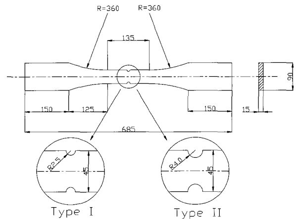
Fig. 2 Configuration of Type I, II Specimen with semi-circular edge notch (unit: mm)
