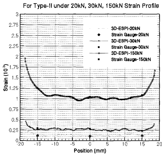
Fig. 6 Strain profile of Type II under 20kN, 30kN, 150kN
