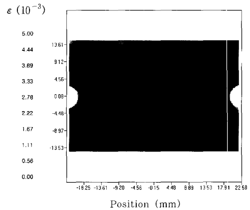
Fig. 3 Strain Distribution of Type I under 150kN
