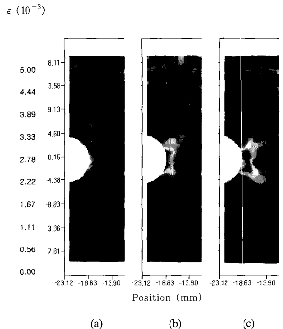
Fig. 10 Change of strain distribution of Type II specimen according to accumulated damage: (a) at 77,787 cycles, (b) at 90,852 cycles, (c) crack initiation at 97,467 cycles
