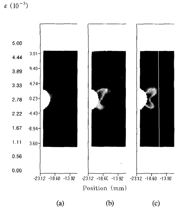
Fig. 9 Change of strain distribution of Type I specimen according to accumulated damage: (a) at 98,872 cycles, (b) at 104,472 cycles, (c) crack initiation at 109,247 cycles
