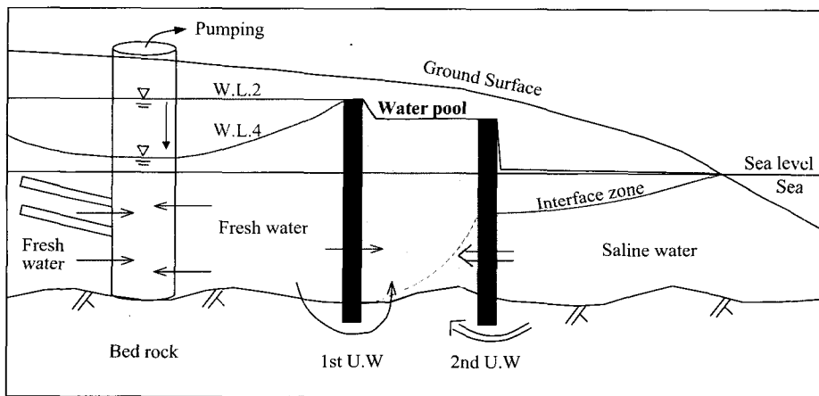
Fig. 4. Two consecutive underground wall to prevent seawater intrusion. (A)Plan view (B)Cross section (U.W. ; Underground Wall, W.L. ; Water Level)
