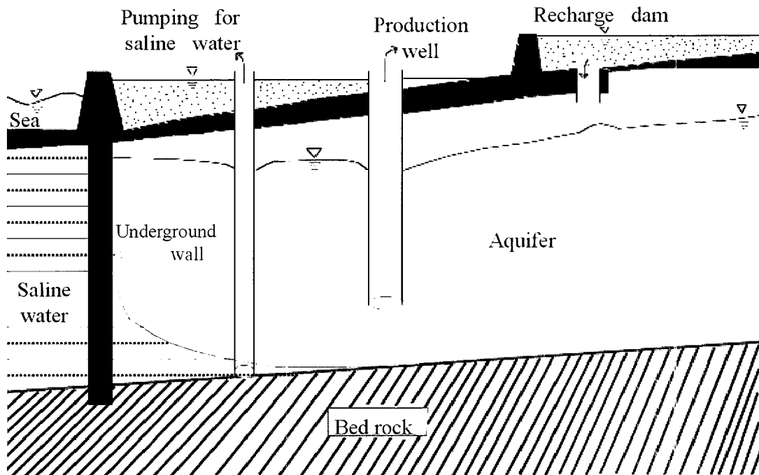
Fig. 1. Schematic cross section of Samganbo groundwater dam
