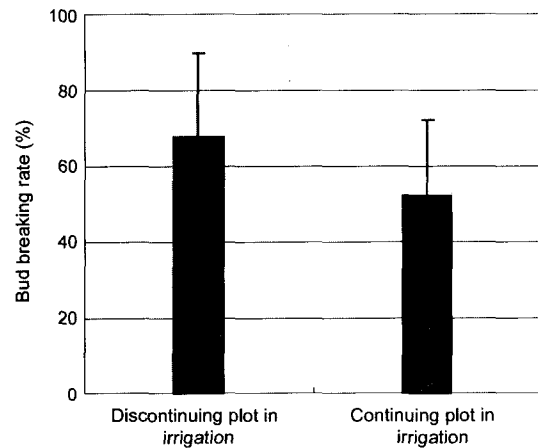
Fig. 1. Comparison of bud breaking rate between the discontinuing plot in irrigation and the continuing plot in irrigation (Bar is standard error. Mean of two years data).
