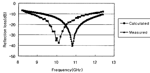
Fig. 5 Measured and calculated reflection loss of the optimal absorbing structure.
