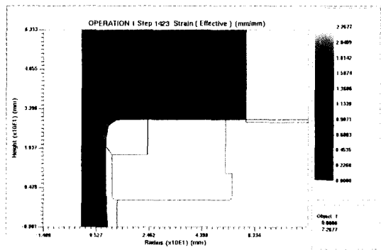
(c) Effective strain distribution
