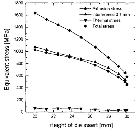
Fig. 8 Equivalent stresses on the height of die insert by total load
