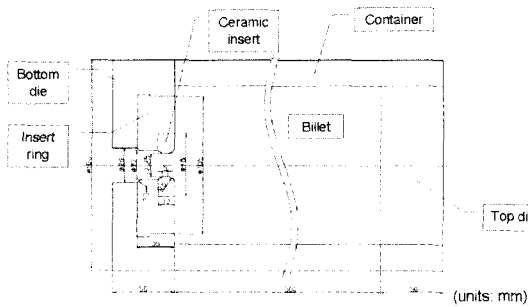
Fig. 2 Tooling system used in hot extrusion process
