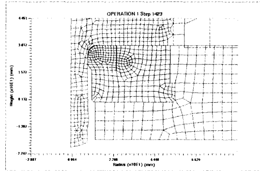
(a) Hot extrusion process
