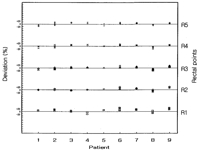
Fig. 3. Distribution of percent in differences between the calculated doses and measured doses [100 (R_m - R_c) / R_c] of each rectal points on rectal diode detector in 9 patients (n=216 rectal points)
