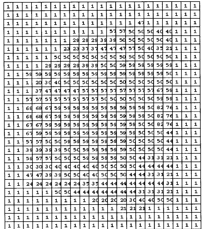
Fig. 2. Intensity map (beam pattern) generated from the Helax RTP system. Higher number indicates the higher dose or longer duration time.
