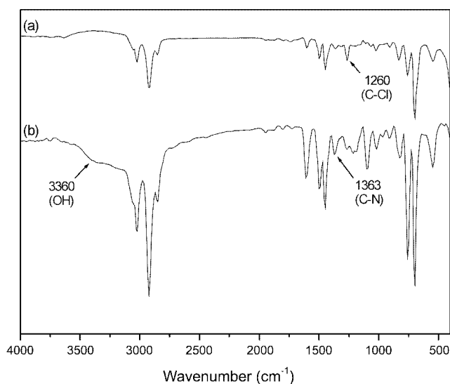
Figure 1. (a) FT-IR spectra of (a) poly(ST-co-VBC) and (b) poly(ST-co-VBC)-DMAP (KBr).
