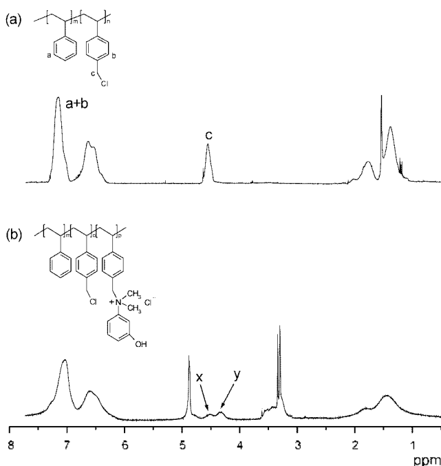
Figure 2. 1 H NMR spectra of (a) poly(ST-co-VBC) (CDCl 3 ) and (b) poly(ST-co-VBC)-DMAP (CD 3 OD).
