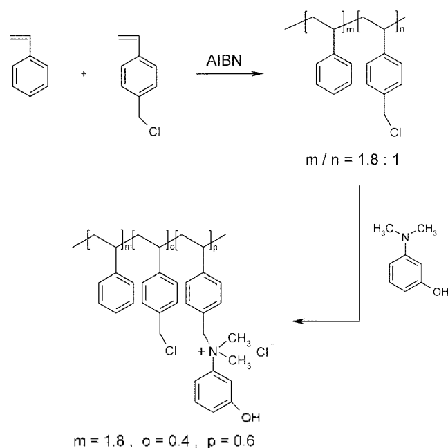
Scheme 1. Synthetic route to poly(ST- co -VBC)-DMAP.
