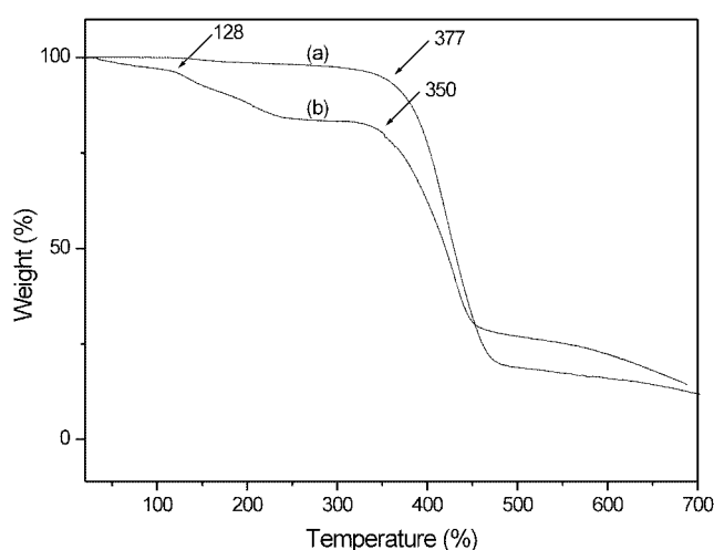
Figure 3. TGA thermograms of (a) poly(ST-co-VBC) and (b) poly(ST-co-VBC)-DMAP. The scanning rate was 20 °C/min.
