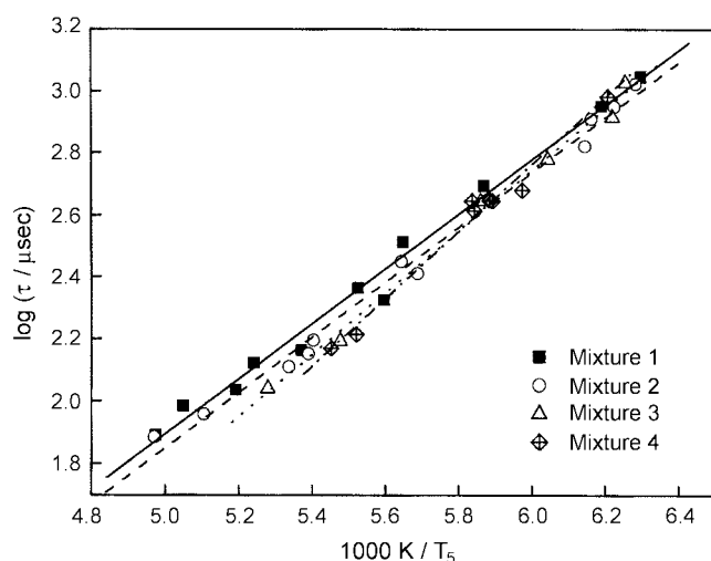
Figure 2. Ignition delay times for the mixtures in Table 1. Lines indicate linear fit for each mixtures.
