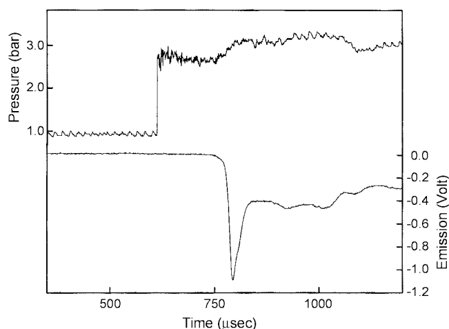
Figure 1. Typical experimental record showing pressure (upper) and OH emission (lower). Experimental conditions were P_1=54 torr and T_5=1763 K in mixture 3.
